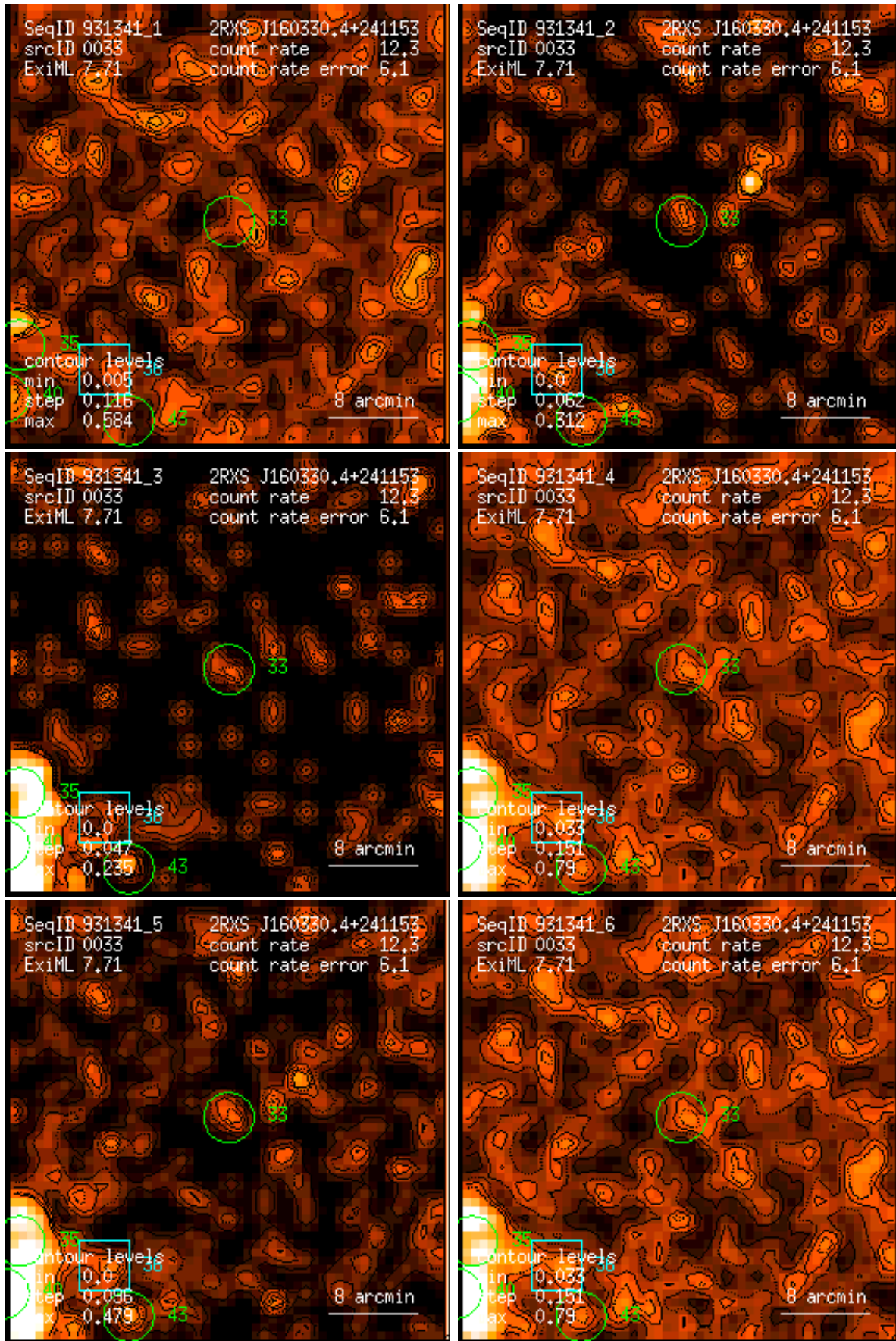
Figure 33: RASS 931341: detection 0033: band rate images, Gaussian filter: (1) PSPC channels 11 – 41, (2) 52 – 90, (3) 91 – 201, (4) 11 – 235, (5) 52 – 201, (6) 11 – 201. Broad band rates in counts/ks. Band rate contour levels in counts/ks/arcmin 2 .
