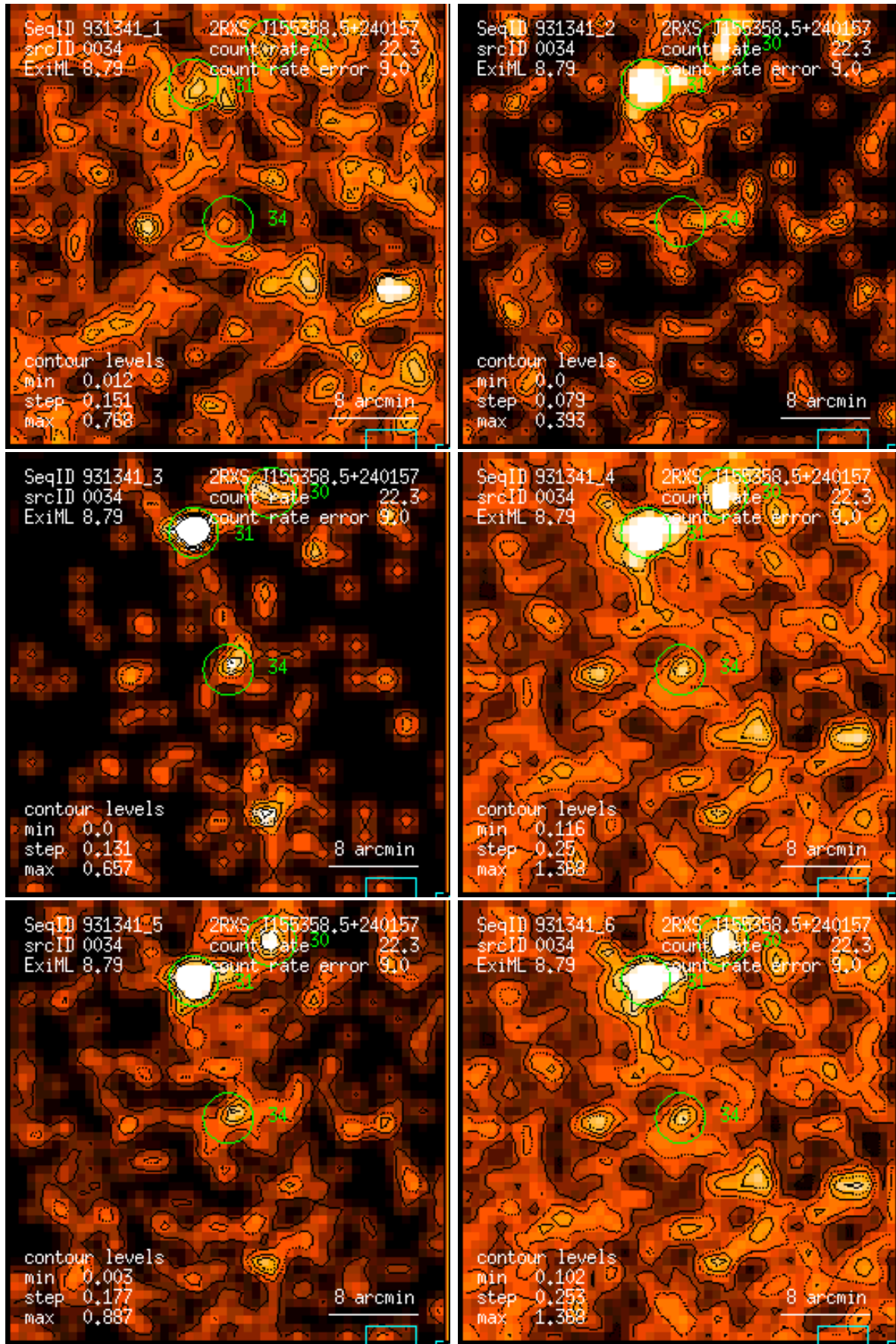
Figure 34: RASS 931341: detection 0034: band rate images, Gaussian filter: (1) PSPC channels 11 – 41, (2) 52 – 90, (3) 91 – 201, (4) 11 – 235, (5) 52 – 201, (6) 11 – 201. Broad band rates in counts/ks. Band rate contour levels in counts/ks/arcmin 2 .
