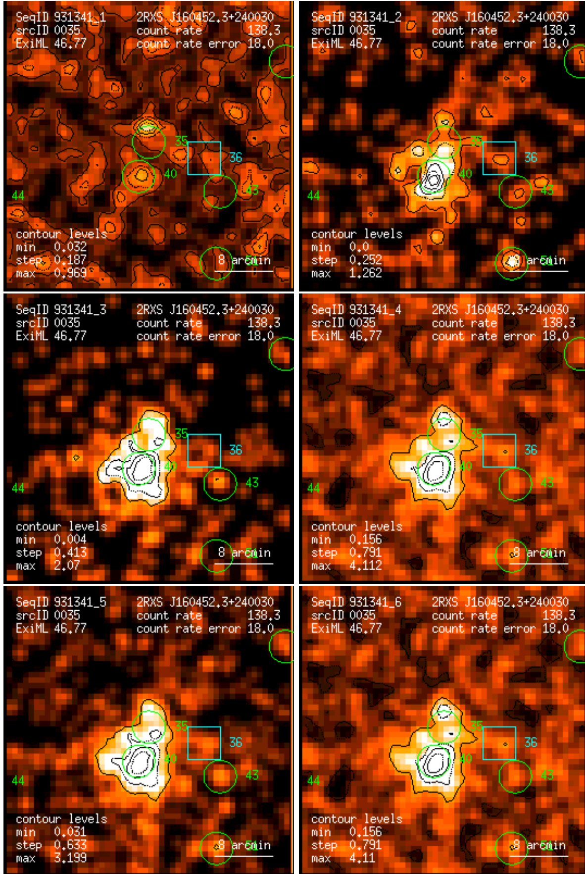
Figure 35: RASS 931341: detection 0035: band rate images, Gaussian filter: (1) PSPC channels 11 – 41, (2) 52 – 90, (3) 91 – 201, (4) 11 – 235, (5) 52 – 201, (6) 11 – 201. Broad band rates in counts/ks. Band rate contour levels in counts/ks/arcmin 2 .
