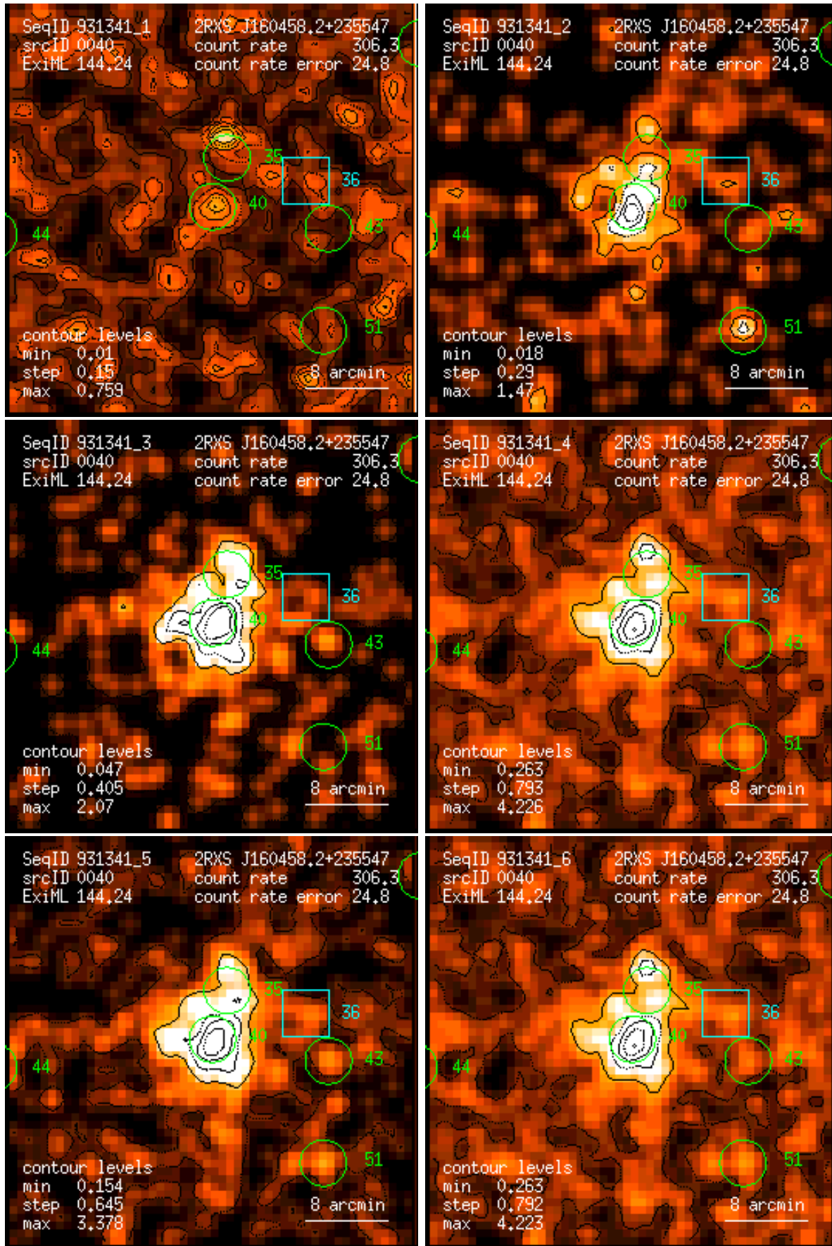
Figure 40: RASS 931341: detection 0040: band rate images, Gaussian filter: (1) PSPC channels 11 – 41, (2) 52 – 90, (3) 91 – 201, (4) 11 – 235, (5) 52 – 201, (6) 11 – 201. Broad band rates in counts/ks. Band rate contour levels in counts/ks/arcmin 2 .
