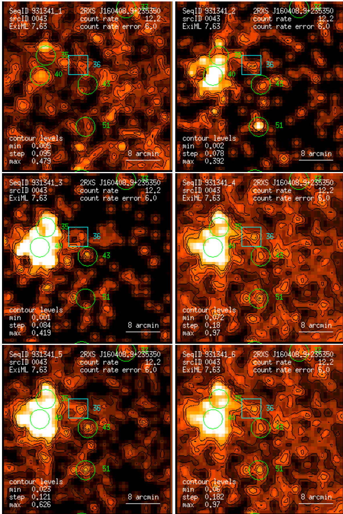
Figure 43: RASS 931341: detection 0043: band rate images, Gaussian filter: (1) PSPC channels 11 – 41, (2) 52 – 90, (3) 91 – 201, (4) 11 – 235, (5) 52 – 201, (6) 11 – 201. Broad band rates in counts/ks. Band rate contour levels in counts/ks/arcmin 2 .
