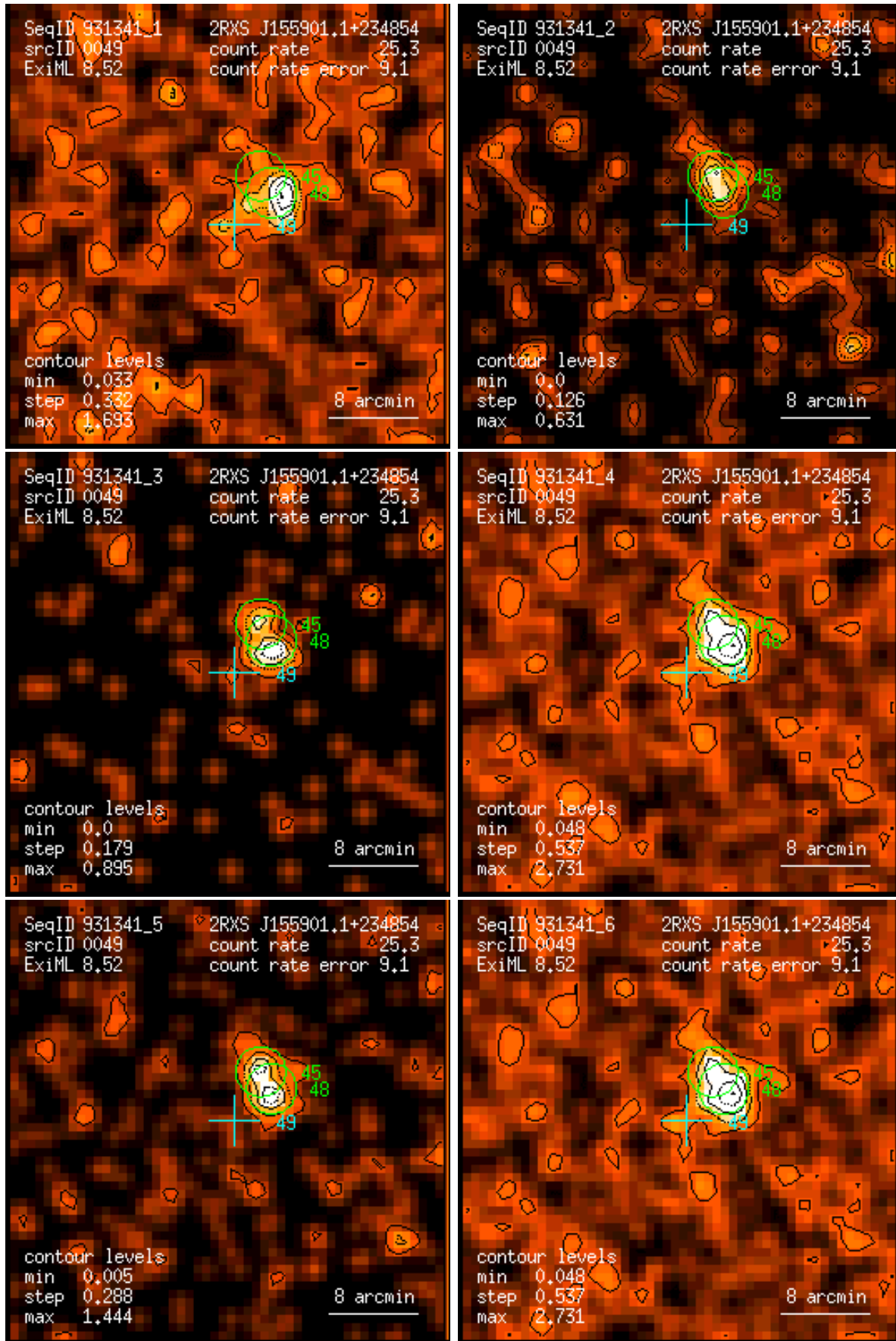
Figure 49: RASS 931341: detection 0049: band rate images, Gaussian filter: (1) PSPC channels 11 – 41, (2) 52 – 90, (3) 91 – 201, (4) 11 – 235, (5) 52 – 201, (6) 11 – 201. Broad band rates in counts/ks. Band rate contour levels in counts/ks/arcmin 2 .
