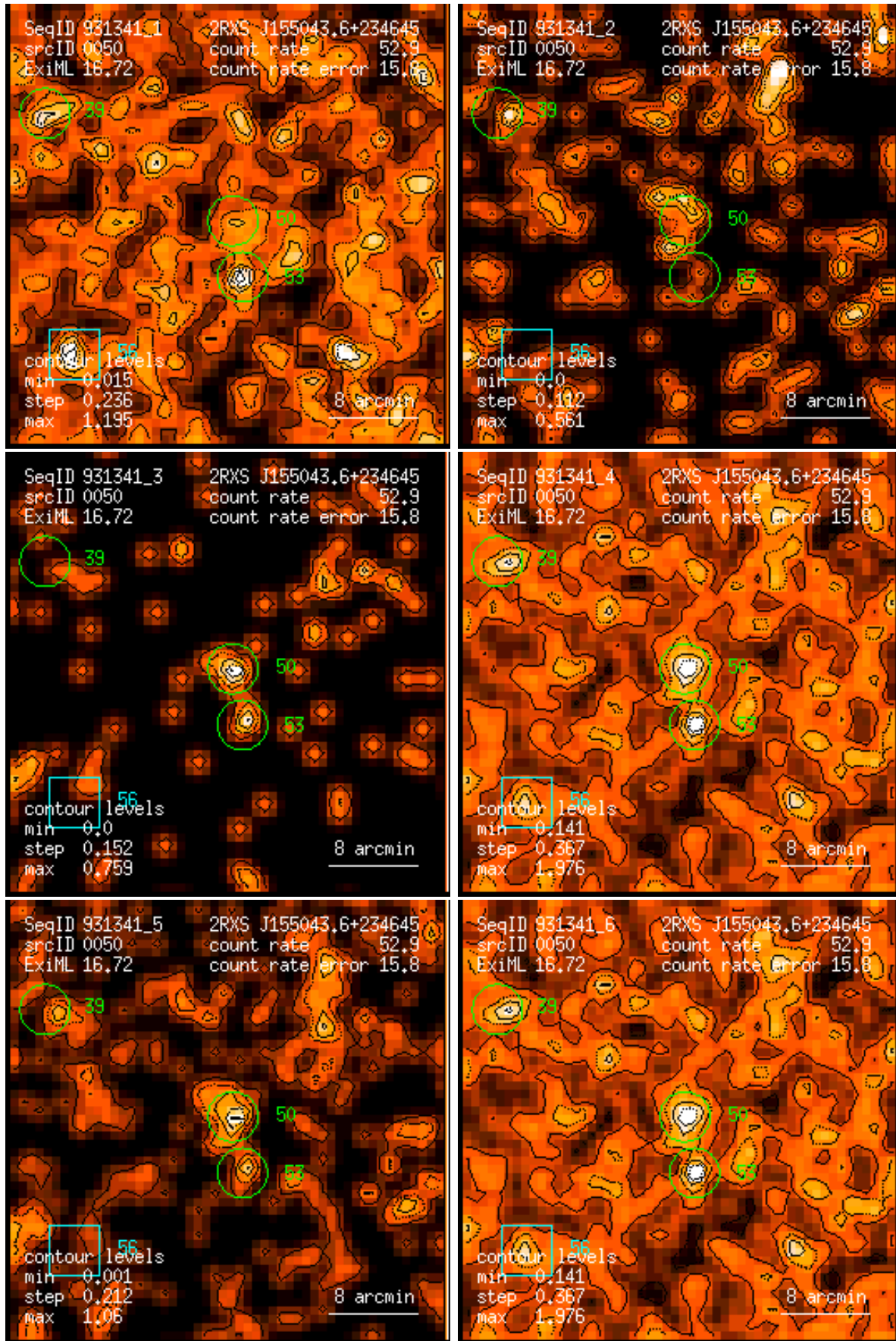
Figure 50: RASS 931341: detection 0050: band rate images, Gaussian filter: (1) PSPC channels 11 – 41, (2) 52 – 90, (3) 91 – 201, (4) 11 – 235, (5) 52 – 201, (6) 11 – 201. Broad band rates in counts/ks. Band rate contour levels in counts/ks/arcmin 2 .
