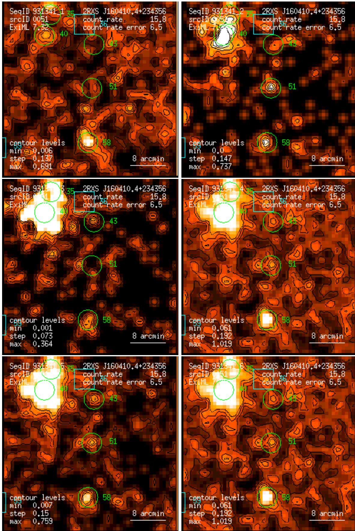
Figure 51: RASS 931341: detection 0051: band rate images, Gaussian filter: (1) PSPC channels 11 – 41, (2) 52 – 90, (3) 91 – 201, (4) 11 – 235, (5) 52 – 201, (6) 11 – 201. Broad band rates in counts/ks. Band rate contour levels in counts/ks/arcmin 2 .
