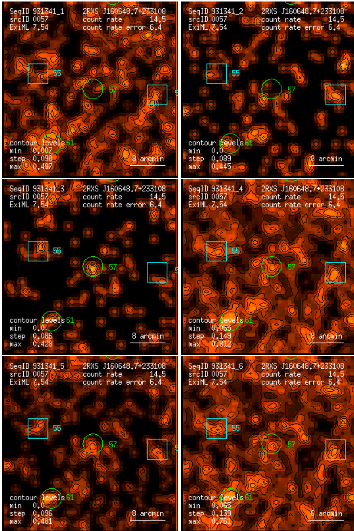
Figure 57: RASS 931341: detection 0057: band rate images, Gaussian filter: (1) PSPC channels 11 – 41, (2) 52 – 90, (3) 91 – 201, (4) 11 – 235, (5) 52 – 201, (6) 11 – 201. Broad band rates in counts/ks. Band rate contour levels in counts/ks/arcmin 2 .
