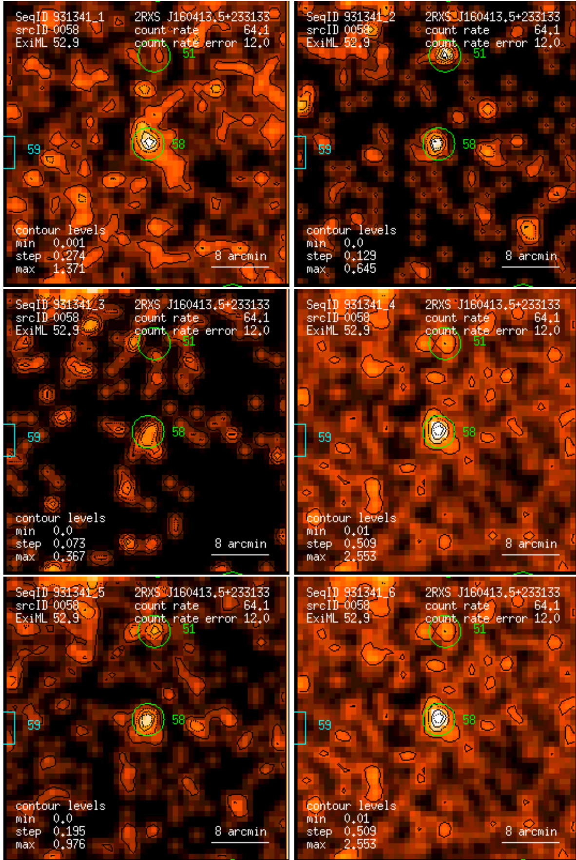
Figure 58: RASS 931341: detection 0058: band rate images, Gaussian filter: (1) PSPC channels 11 – 41, (2) 52 – 90, (3) 91 – 201, (4) 11 – 235, (5) 52 – 201, (6) 11 – 201. Broad band rates in counts/ks. Band rate contour levels in counts/ks/arcmin 2 .
