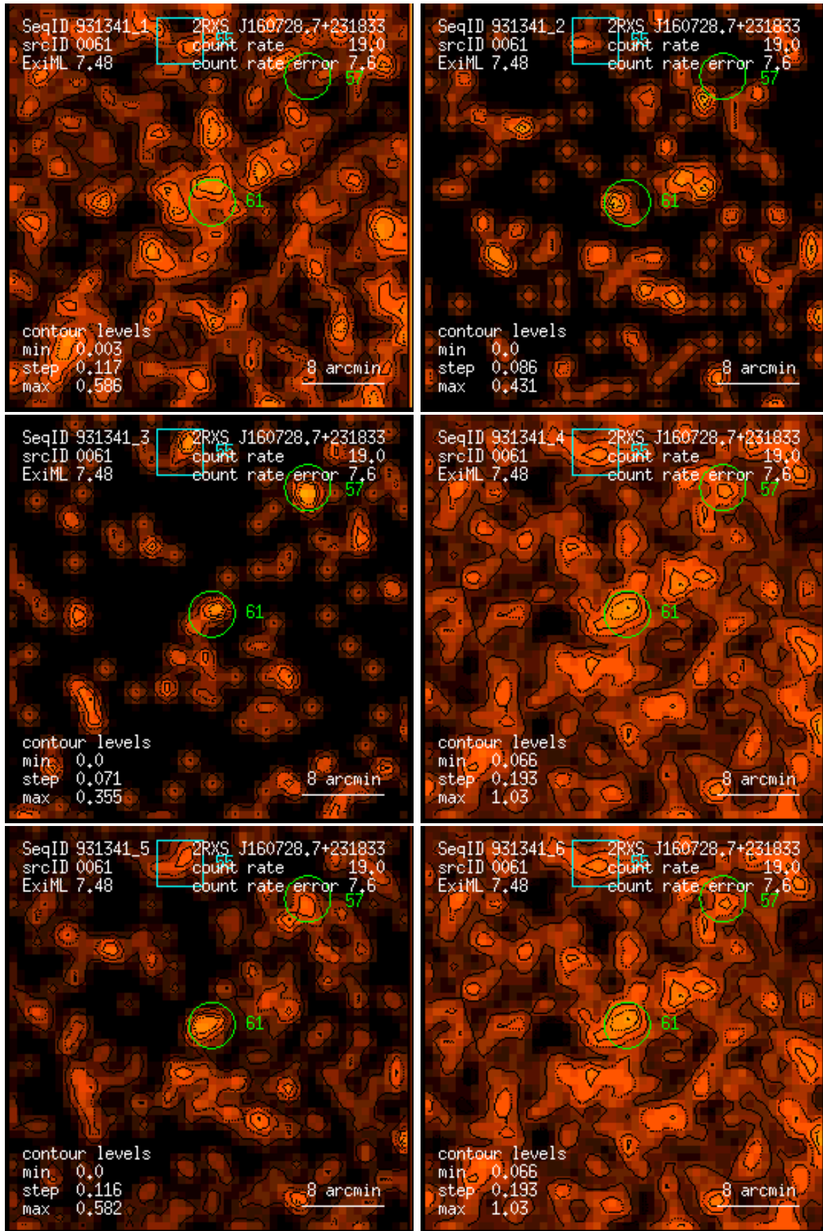
Figure 61: RASS 931341: detection 0061: band rate images, Gaussian filter: (1) PSPC channels 11 – 41, (2) 52 – 90, (3) 91 – 201, (4) 11 – 235, (5) 52 – 201, (6) 11 – 201. Broad band rates in counts/ks. Band rate contour levels in counts/ks/arcmin 2 .
