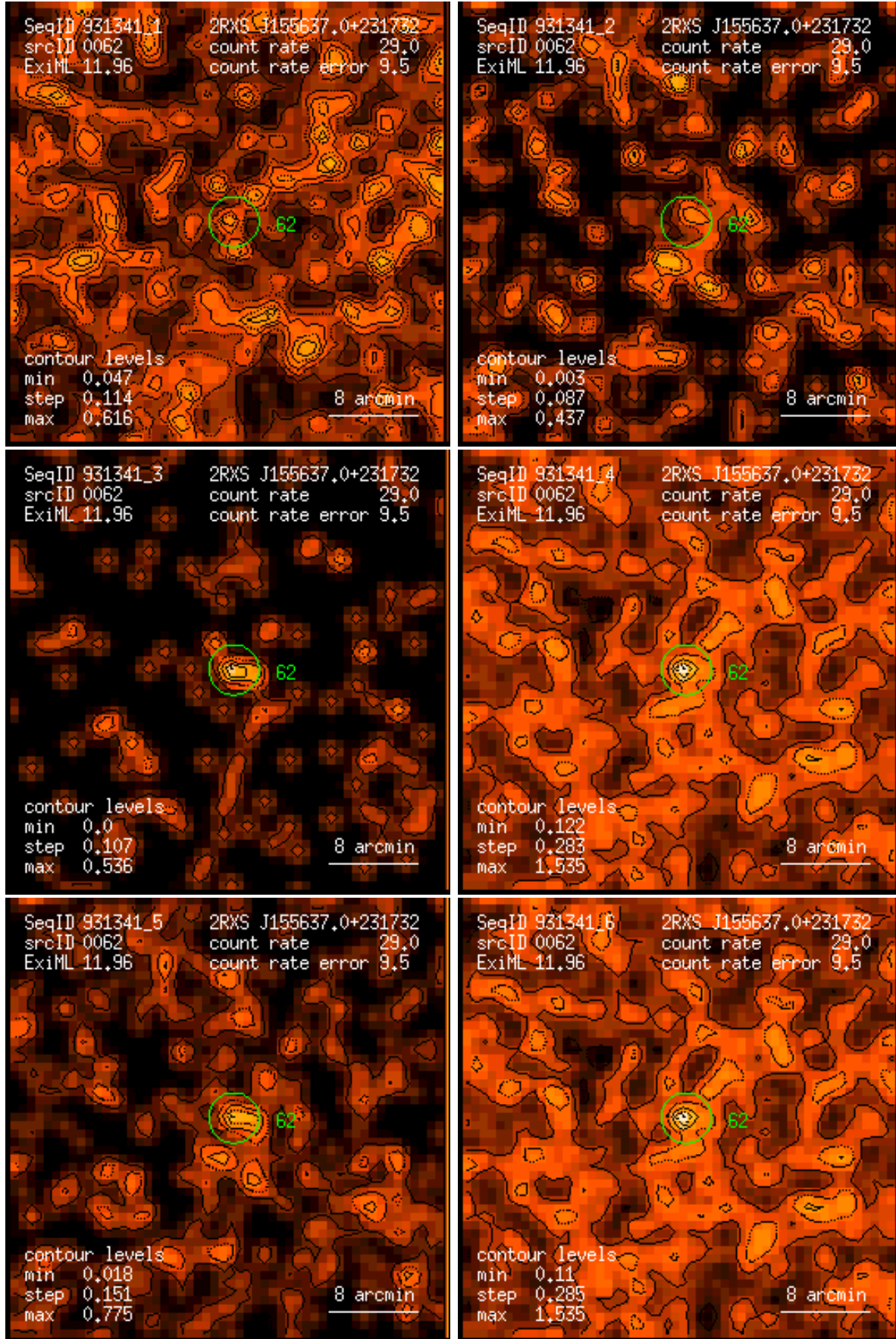
Figure 62: RASS 931341: detection 0062: band rate images, Gaussian filter: (1) PSPC channels 11 – 41, (2) 52 – 90, (3) 91 – 201, (4) 11 – 235, (5) 52 – 201, (6) 11 – 201. Broad band rates in counts/ks. Band rate contour levels in counts/ks/arcmin 2 .
