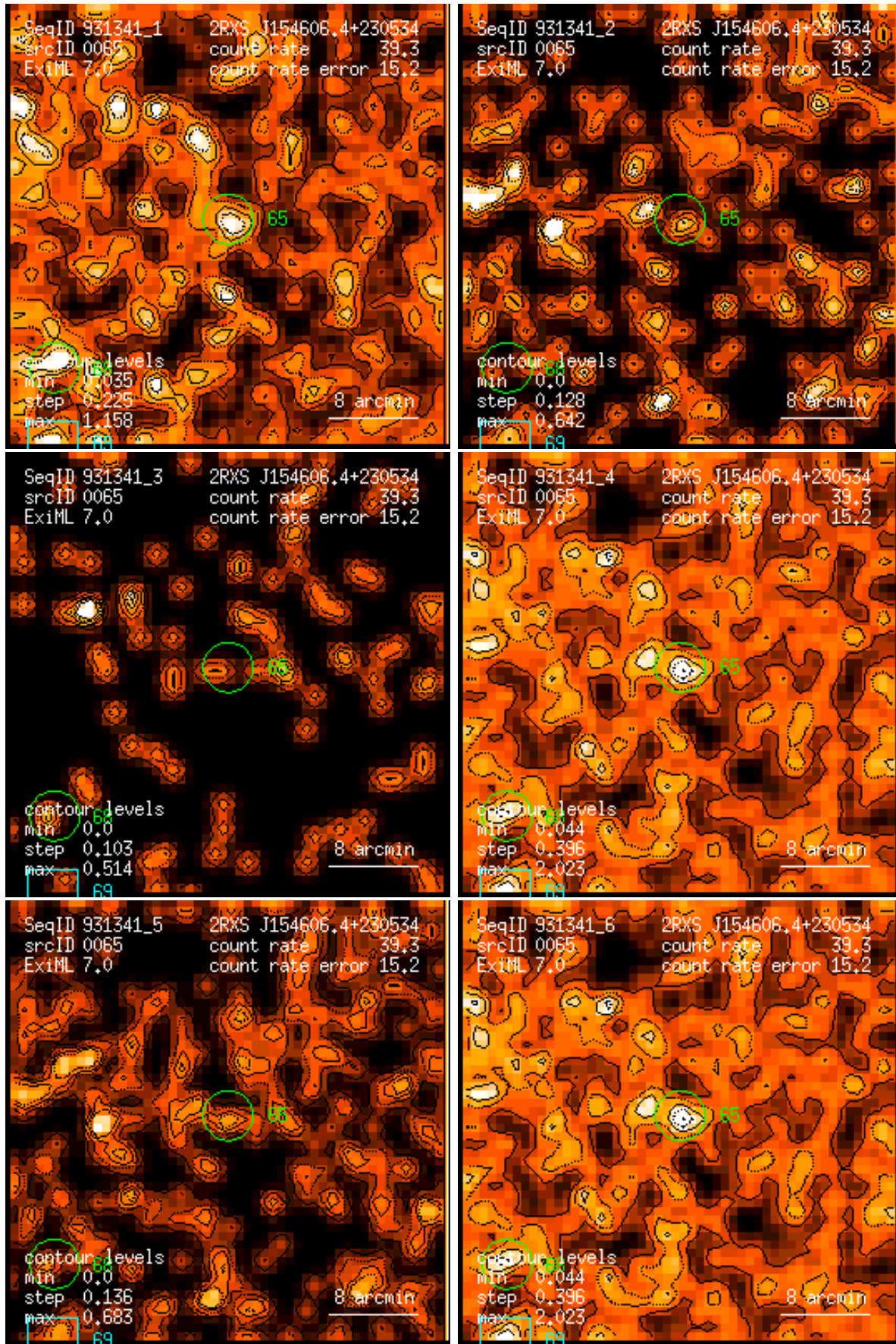
Figure 65: RASS 931341: detection 0065: band rate images, Gaussian filter: (1) PSPC channels 11 – 41, (2) 52 – 90, (3) 91 – 201, (4) 11 – 235, (5) 52 – 201, (6) 11 – 201. Broad band rates in counts/ks. Band rate contour levels in counts/ks/arcmin 2 .
