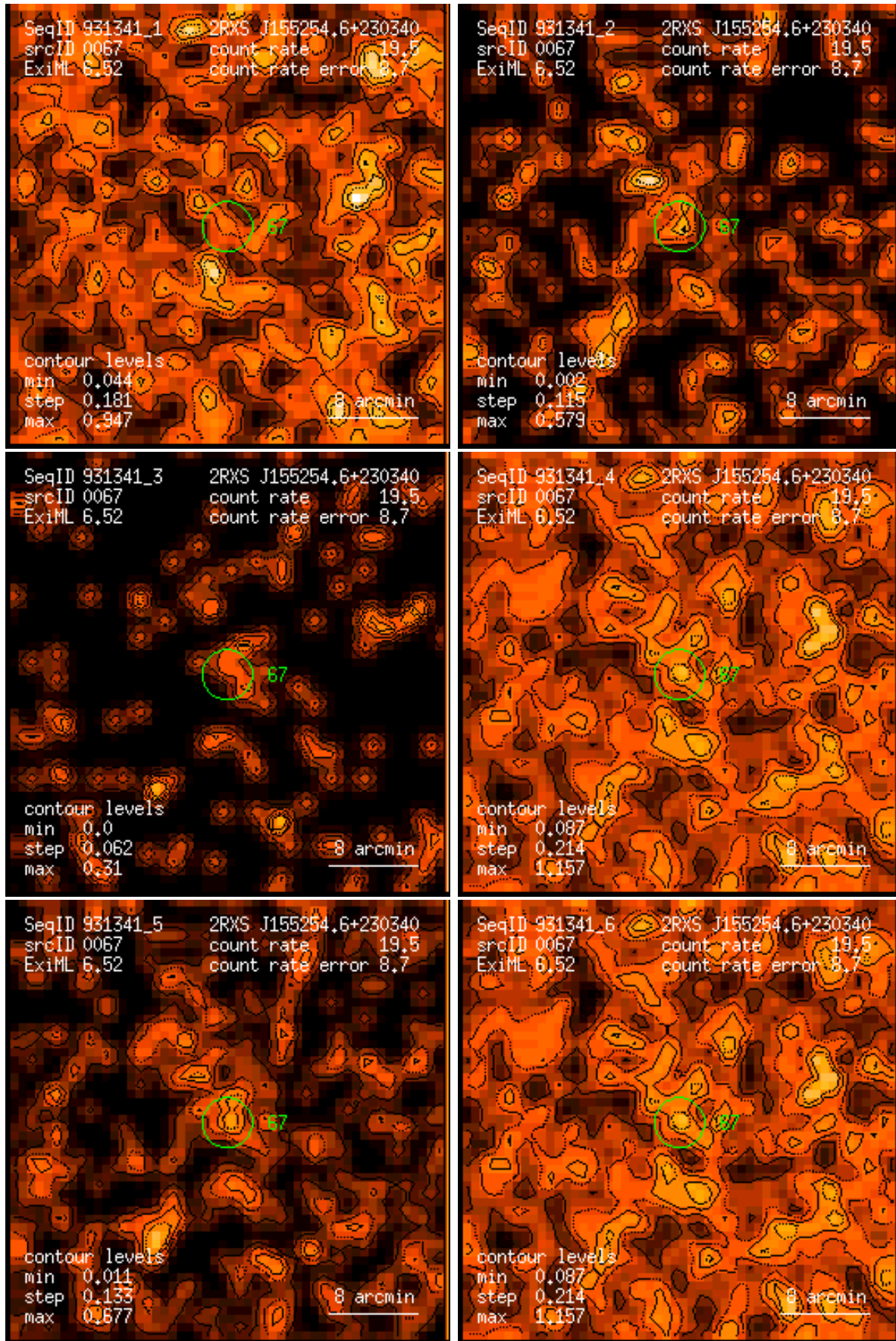
Figure 67: RASS 931341: detection 0067: band rate images, Gaussian filter: (1) PSPC channels 11 – 41, (2) 52 – 90, (3) 91 – 201, (4) 11 – 235, (5) 52 – 201, (6) 11 – 201. Broad band rates in counts/ks. Band rate contour levels in counts/ks/arcmin 2 .
