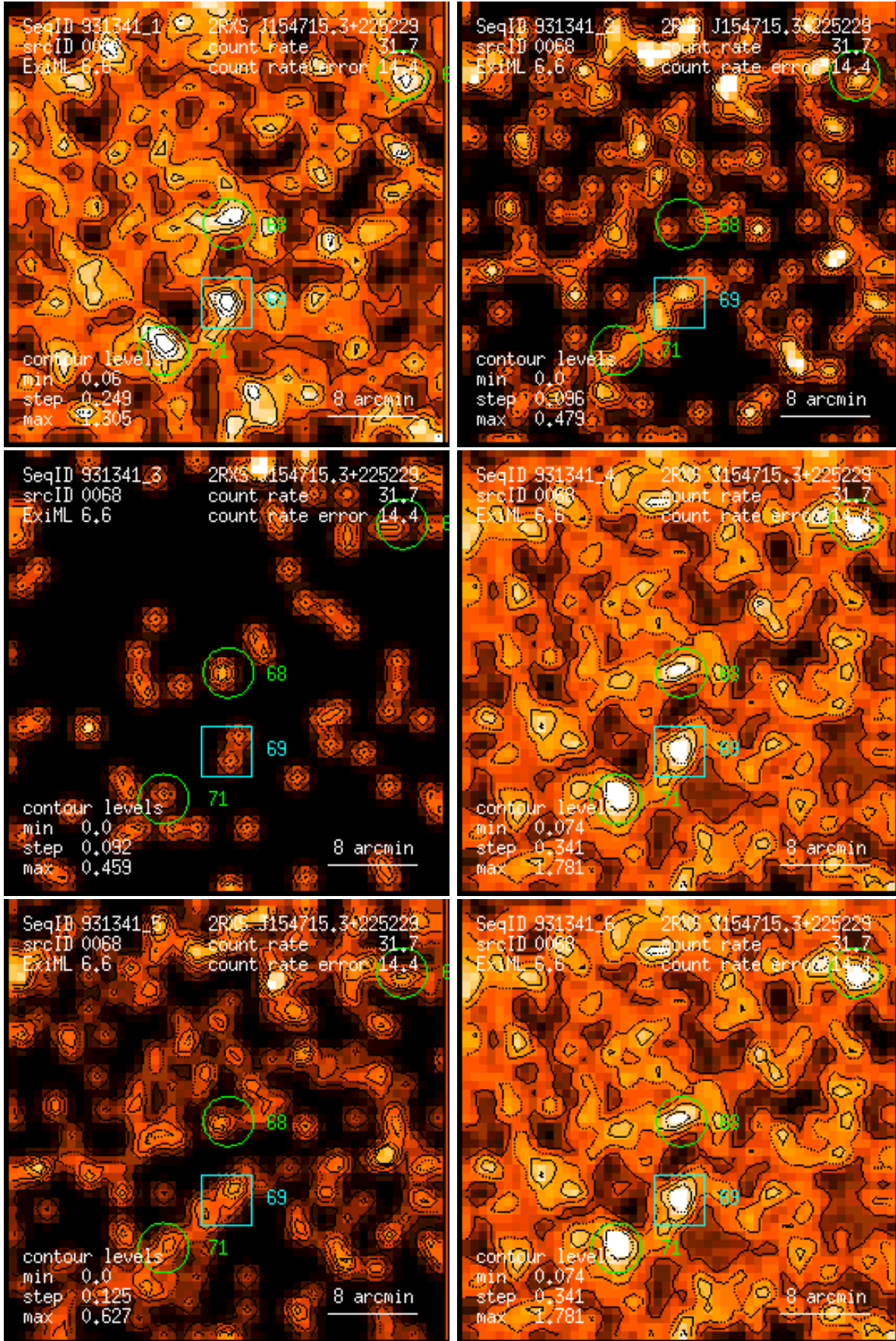
Figure 68: RASS 931341: detection 0068: band rate images, Gaussian filter: (1) PSPC channels 11 – 41, (2) 52 – 90, (3) 91 – 201, (4) 11 – 235, (5) 52 – 201, (6) 11 – 201. Broad band rates in counts/ks. Band rate contour levels in counts/ks/arcmin 2 .
