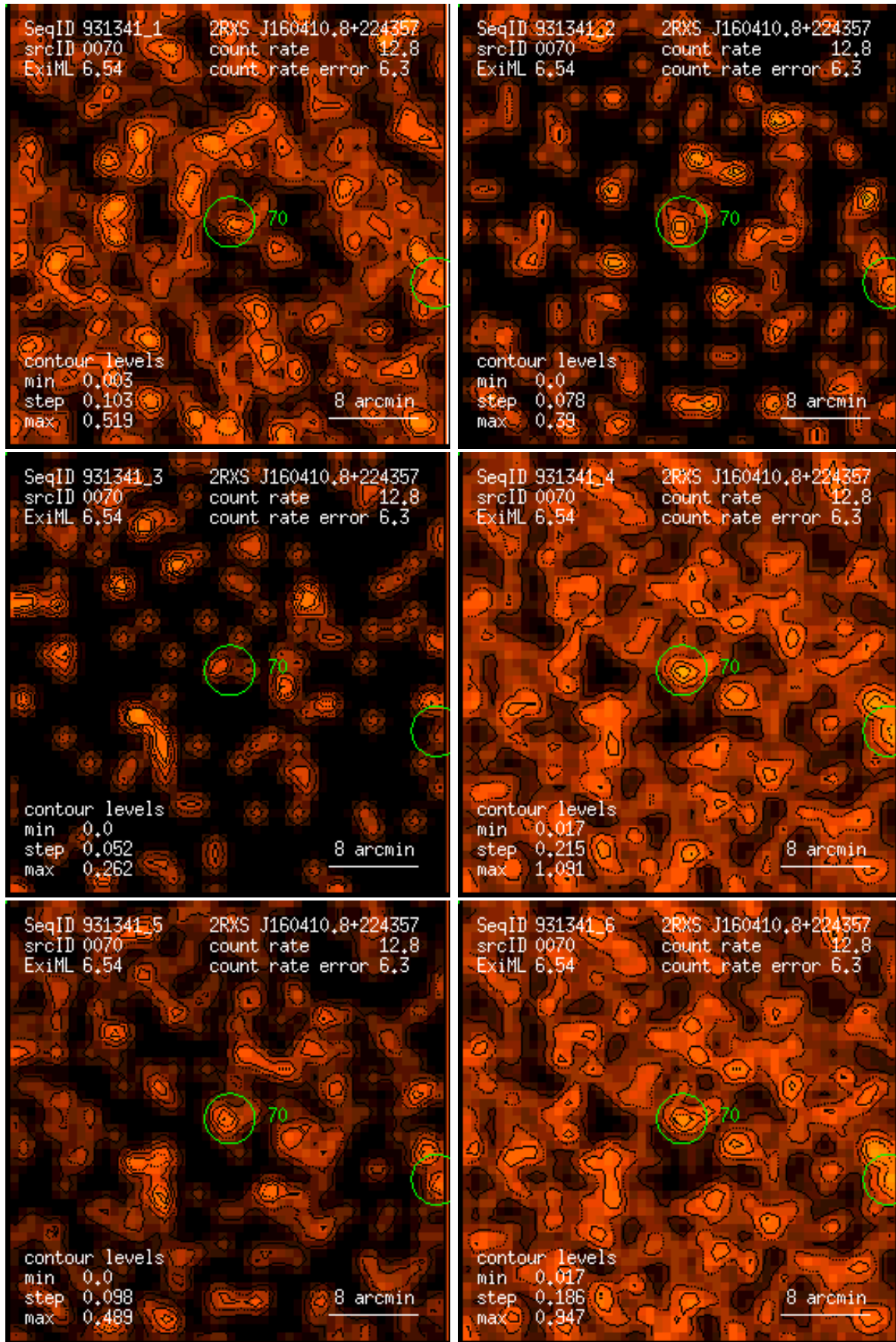
Figure 70: RASS 931341: detection 0070: band rate images, Gaussian filter: (1) PSPC channels 11 – 41, (2) 52 – 90, (3) 91 – 201, (4) 11 – 235, (5) 52 – 201, (6) 11 – 201. Broad band rates in counts/ks. Band rate contour levels in counts/ks/arcmin 2 .
