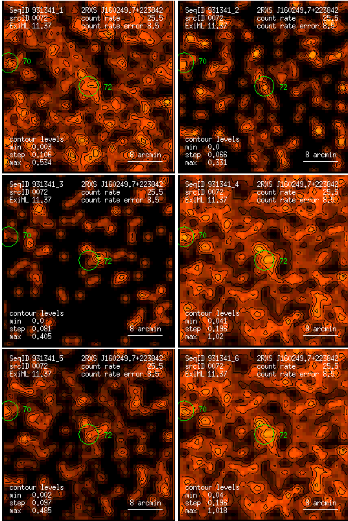
Figure 72: RASS 931341: detection 0072: band rate images, Gaussian filter: (1) PSPC channels 11 – 41, (2) 52 – 90, (3) 91 – 201, (4) 11 – 235, (5) 52 – 201, (6) 11 – 201. Broad band rates in counts/ks. Band rate contour levels in counts/ks/arcmin 2 .
