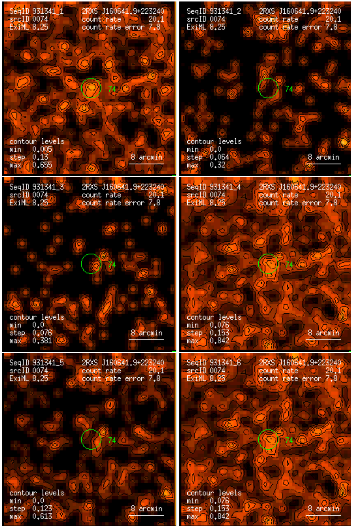
Figure 74: RASS 931341: detection 0074: band rate images, Gaussian filter: (1) PSPC channels 11 – 41, (2) 52 – 90, (3) 91 – 201, (4) 11 – 235, (5) 52 – 201, (6) 11 – 201. Broad band rates in counts/ks. Band rate contour levels in counts/ks/arcmin 2 .
