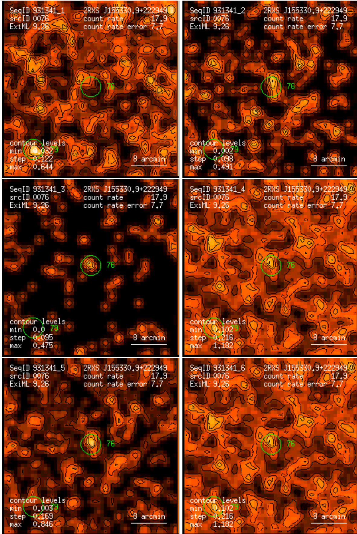
Figure 76: RASS 931341: detection 0076: band rate images, Gaussian filter: (1) PSPC channels 11 – 41, (2) 52 – 90, (3) 91 – 201, (4) 11 – 235, (5) 52 – 201, (6) 11 – 201. Broad band rates in counts/ks. Band rate contour levels in counts/ks/arcmin 2 .
