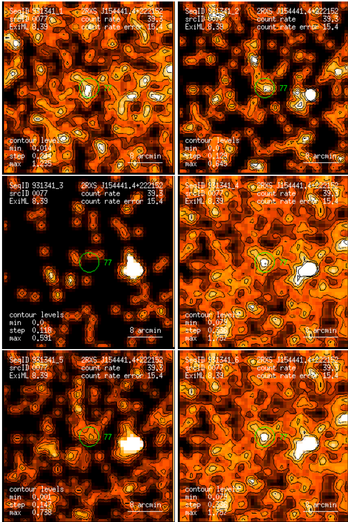
Figure 77: RASS 931341: detection 0077: band rate images, Gaussian filter: (1) PSPC channels 11 – 41, (2) 52 – 90, (3) 91 – 201, (4) 11 – 235, (5) 52 – 201, (6) 11 – 201. Broad band rates in counts/ks. Band rate contour levels in counts/ks/arcmin 2 .
