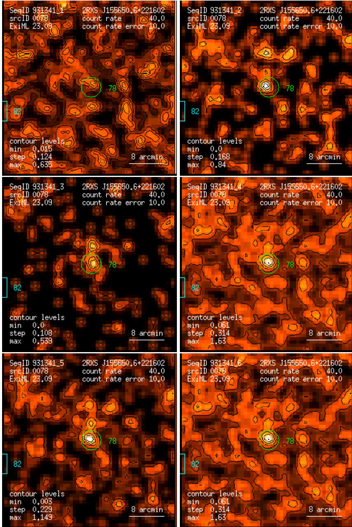
Figure 78: RASS 931341: detection 0078: band rate images, Gaussian filter: (1) PSPC channels 11 – 41, (2) 52 – 90, (3) 91 – 201, (4) 11 – 235, (5) 52 – 201, (6) 11 – 201. Broad band rates in counts/ks. Band rate contour levels in counts/ks/arcmin 2 .
