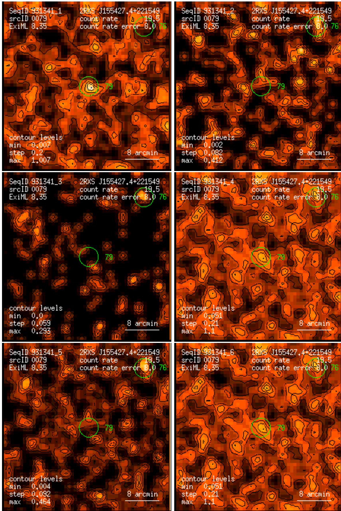
Figure 79: RASS 931341: detection 0079: band rate images, Gaussian filter: (1) PSPC channels 11 – 41, (2) 52 – 90, (3) 91 – 201, (4) 11 – 235, (5) 52 – 201, (6) 11 – 201. Broad band rates in counts/ks. Band rate contour levels in counts/ks/arcmin 2 .
