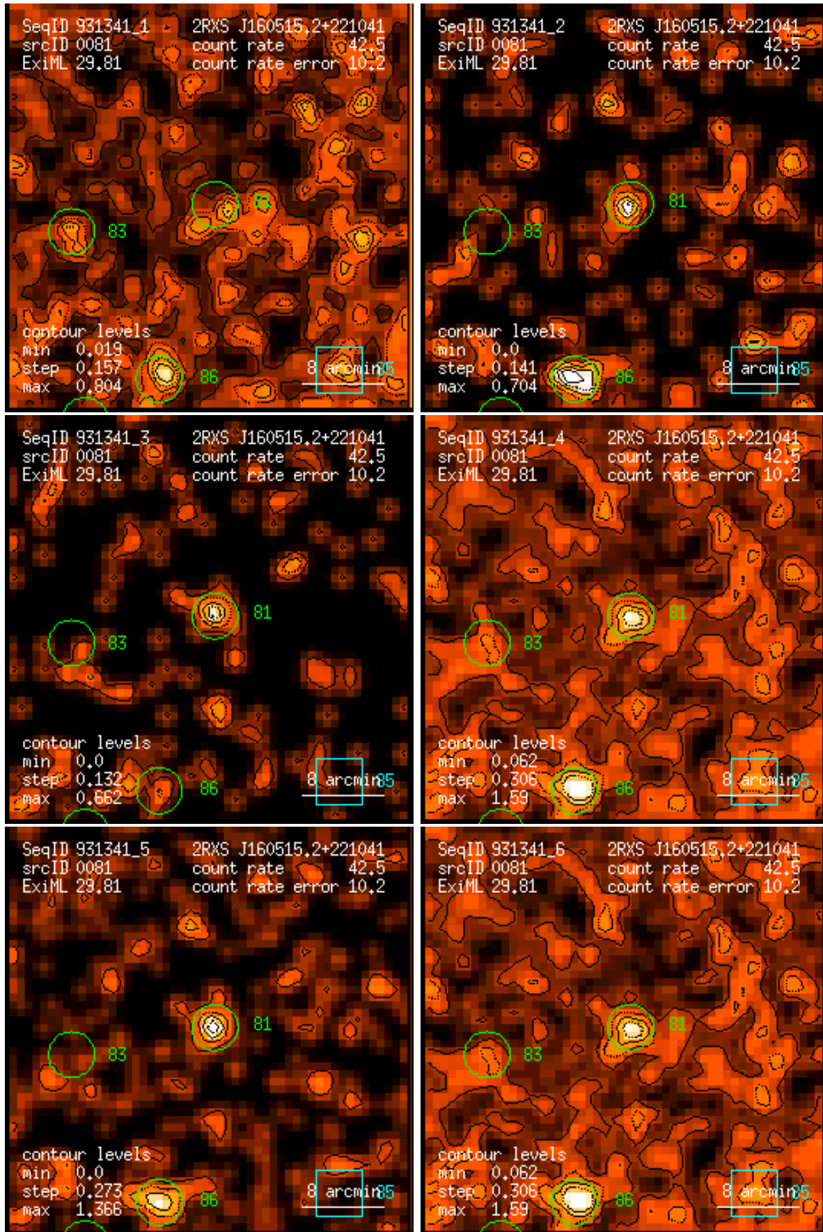
Figure 81: RASS 931341: detection 0081: band rate images, Gaussian filter: (1) PSPC channels 11 – 41, (2) 52 – 90, (3) 91 – 201, (4) 11 – 235, (5) 52 – 201, (6) 11 – 201. Broad band rates in counts/ks. Band rate contour levels in counts/ks/arcmin 2 .
