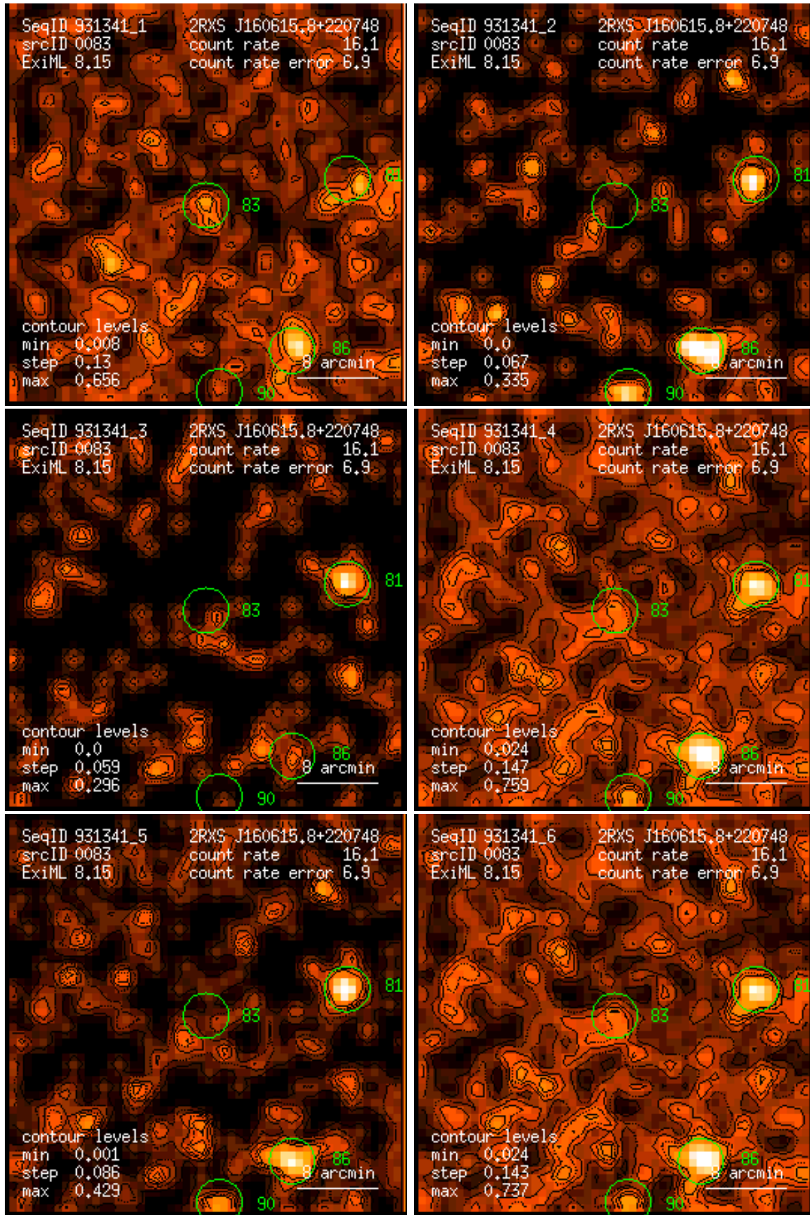
Figure 83: RASS 931341: detection 0083: band rate images, Gaussian filter: (1) PSPC channels 11 – 41, (2) 52 – 90, (3) 91 – 201, (4) 11 – 235, (5) 52 – 201, (6) 11 – 201. Broad band rates in counts/ks. Band rate contour levels in counts/ks/arcmin 2 .
