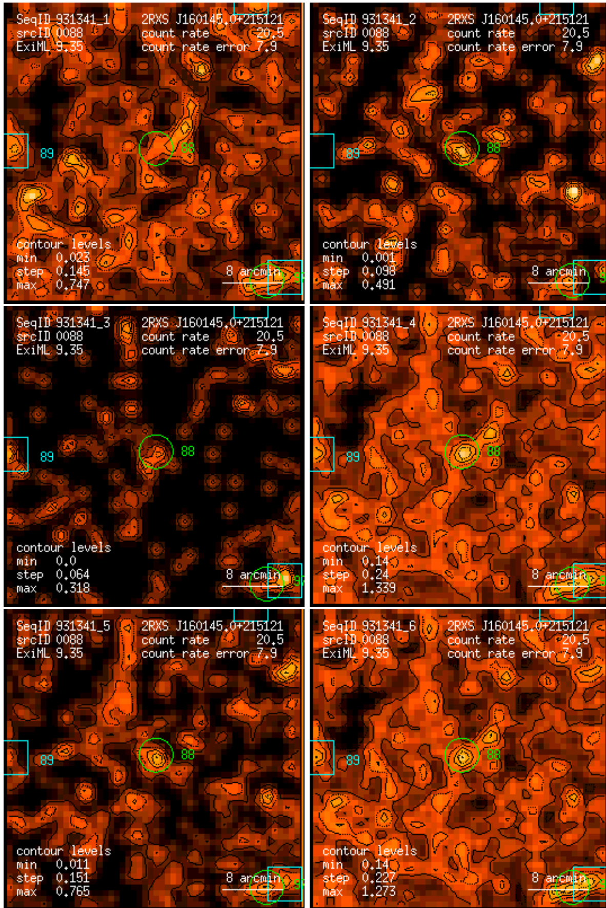
Figure 88: RASS 931341: detection 0088: band rate images, Gaussian filter: (1) PSPC channels 11 – 41, (2) 52 – 90, (3) 91 – 201, (4) 11 – 235, (5) 52 – 201, (6) 11 – 201. Broad band rates in counts/ks. Band rate contour levels in counts/ks/arcmin 2 .
