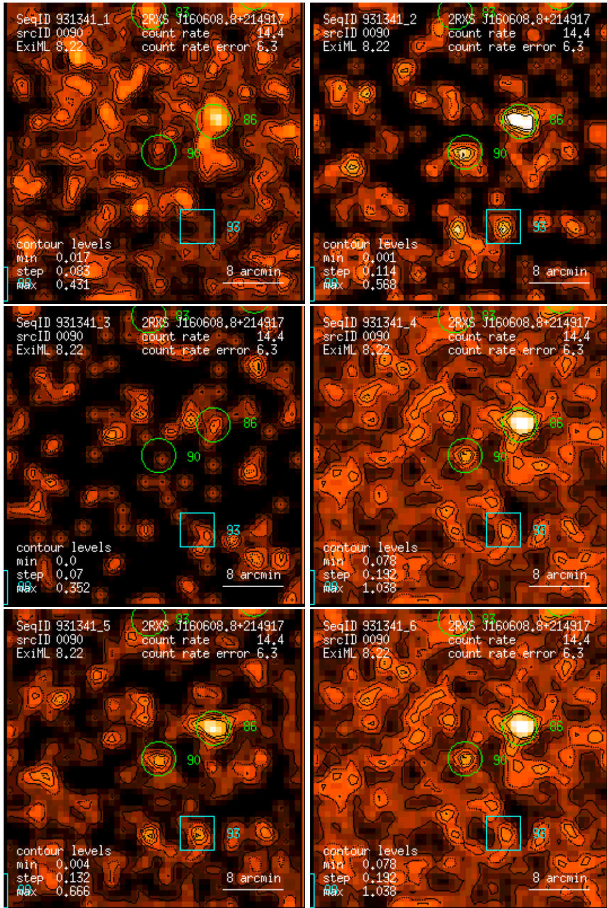
Figure 90: RASS 931341: detection 0090: band rate images, Gaussian filter: (1) PSPC channels 11 – 41, (2) 52 – 90, (3) 91 – 201, (4) 11 – 235, (5) 52 – 201, (6) 11 – 201. Broad band rates in counts/ks. Band rate contour levels in counts/ks/arcmin 2 .
