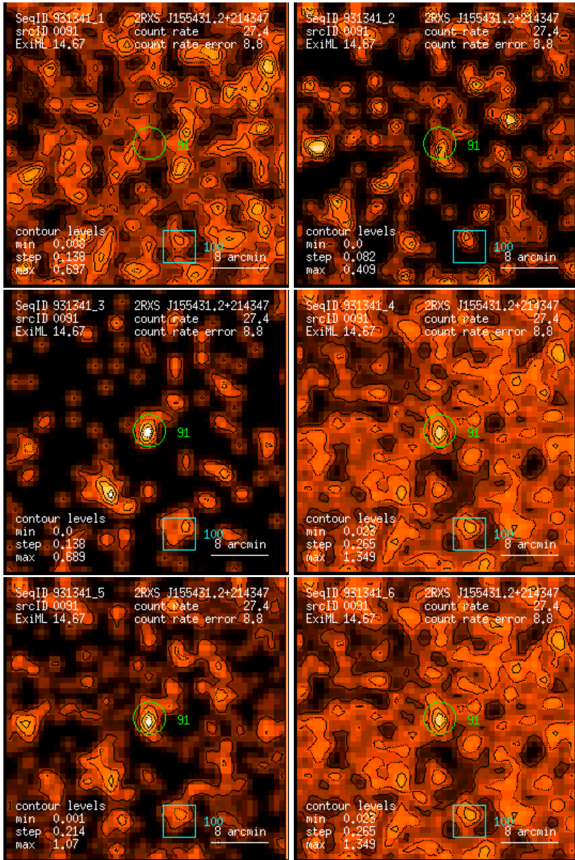
Figure 91: RASS 931341: detection 0091: band rate images, Gaussian filter: (1) PSPC channels 11 – 41, (2) 52 – 90, (3) 91 – 201, (4) 11 – 235, (5) 52 – 201, (6) 11 – 201. Broad band rates in counts/ks. Band rate contour levels in counts/ks/arcmin 2 .
