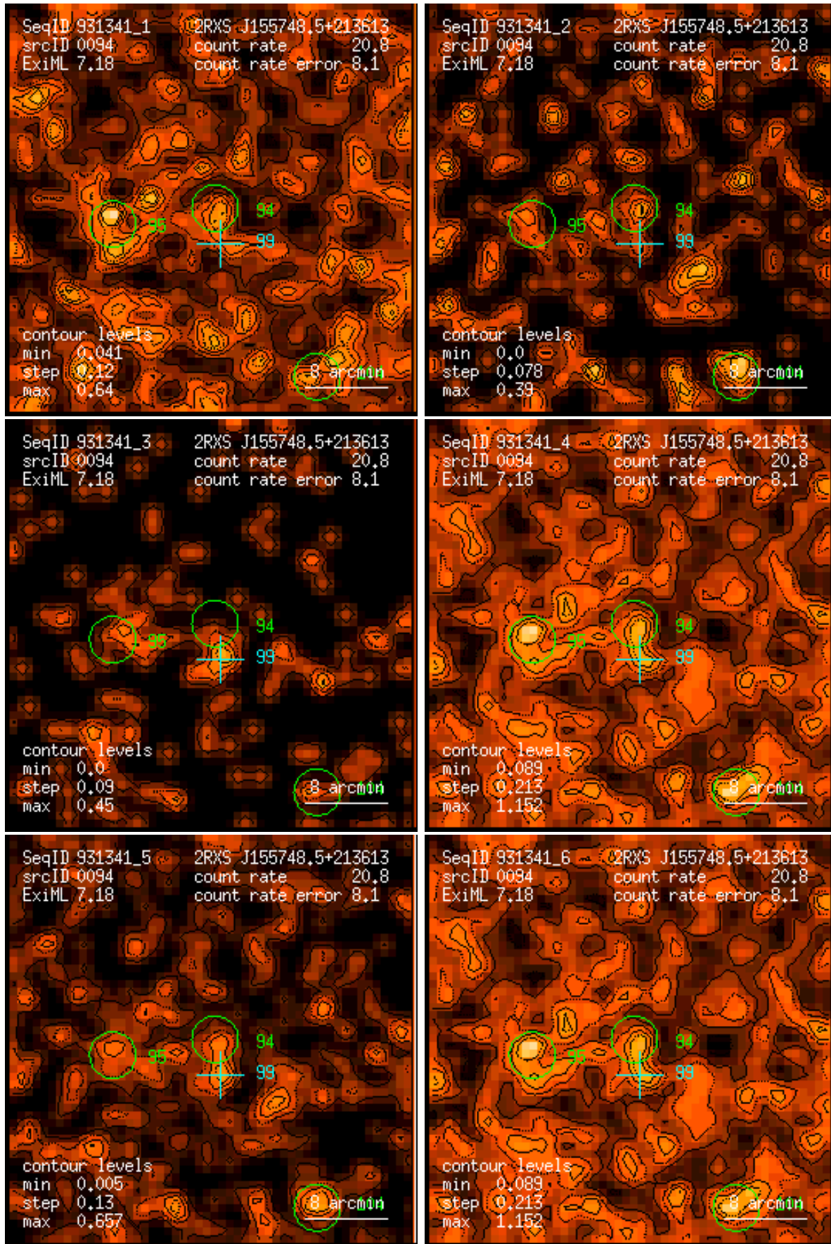
Figure 94: RASS 931341: detection 0094: band rate images, Gaussian filter: (1) PSPC channels 11 – 41, (2) 52 – 90, (3) 91 – 201, (4) 11 – 235, (5) 52 – 201, (6) 11 – 201. Broad band rates in counts/ks. Band rate contour levels in counts/ks/arcmin 2 .
