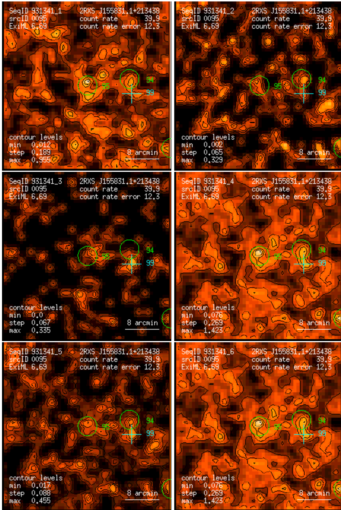
Figure 95: RASS 931341: detection 0095: band rate images, Gaussian filter: (1) PSPC channels 11 – 41, (2) 52 – 90, (3) 91 – 201, (4) 11 – 235, (5) 52 – 201, (6) 11 – 201. Broad band rates in counts/ks. Band rate contour levels in counts/ks/arcmin 2 .
