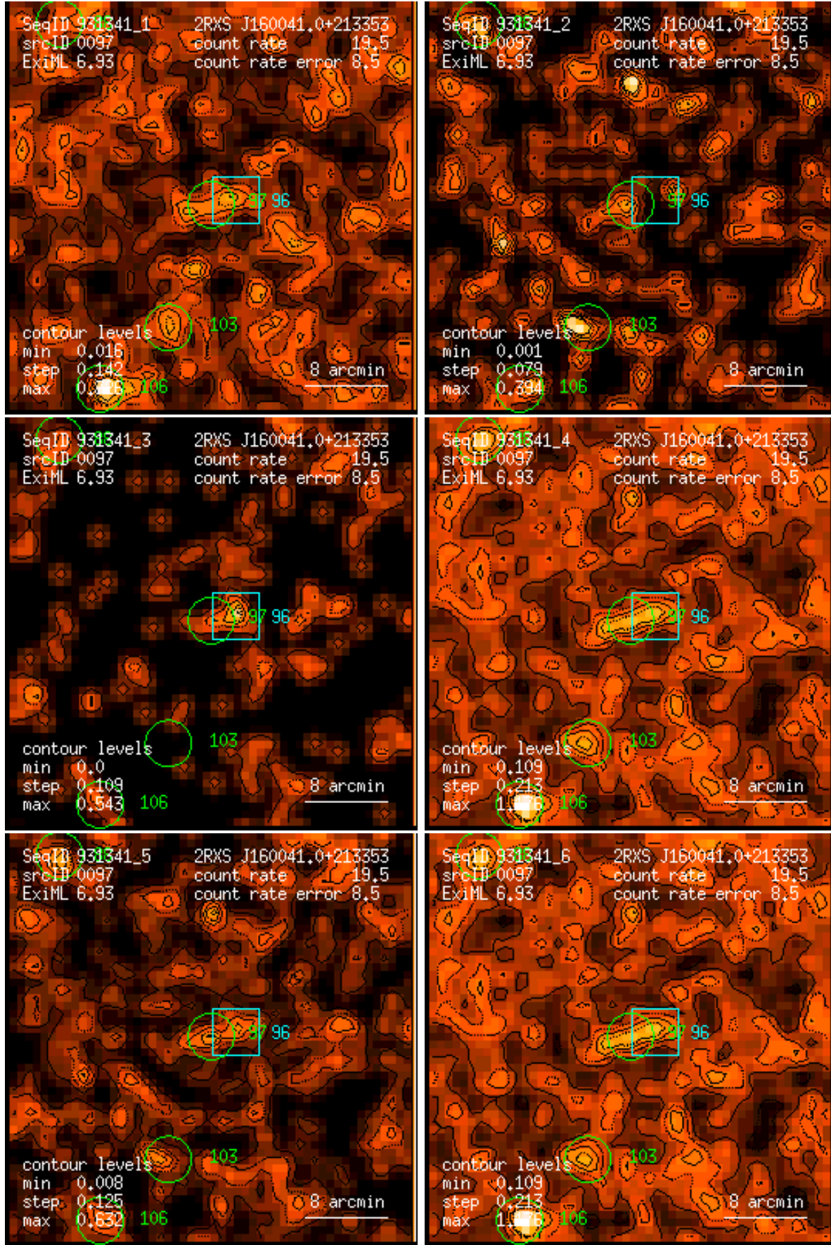
Figure 97: RASS 931341: detection 0097: band rate images, Gaussian filter: (1) PSPC channels 11 – 41, (2) 52 – 90, (3) 91 – 201, (4) 11 – 235, (5) 52 – 201, (6) 11 – 201. Broad band rates in counts/ks. Band rate contour levels in counts/ks/arcmin 2 .
