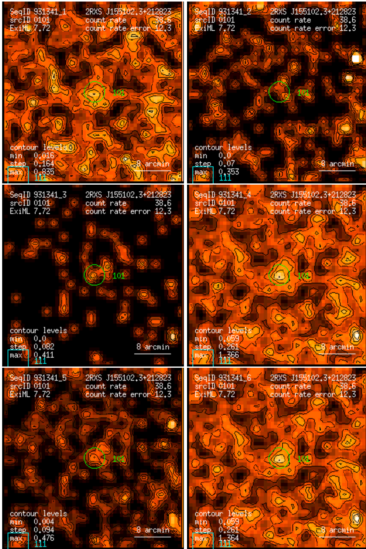
Figure 101: RASS 931341: detection 0101: band rate images, Gaussian filter: (1) PSPC channels 11 – 41, (2) 52 – 90, (3) 91 – 201, (4) 11 – 235, (5) 52 – 201, (6) 11 – 201. Broad band rates in counts/ks. Band rate contour levels in counts/ks/arcmin 2 .
