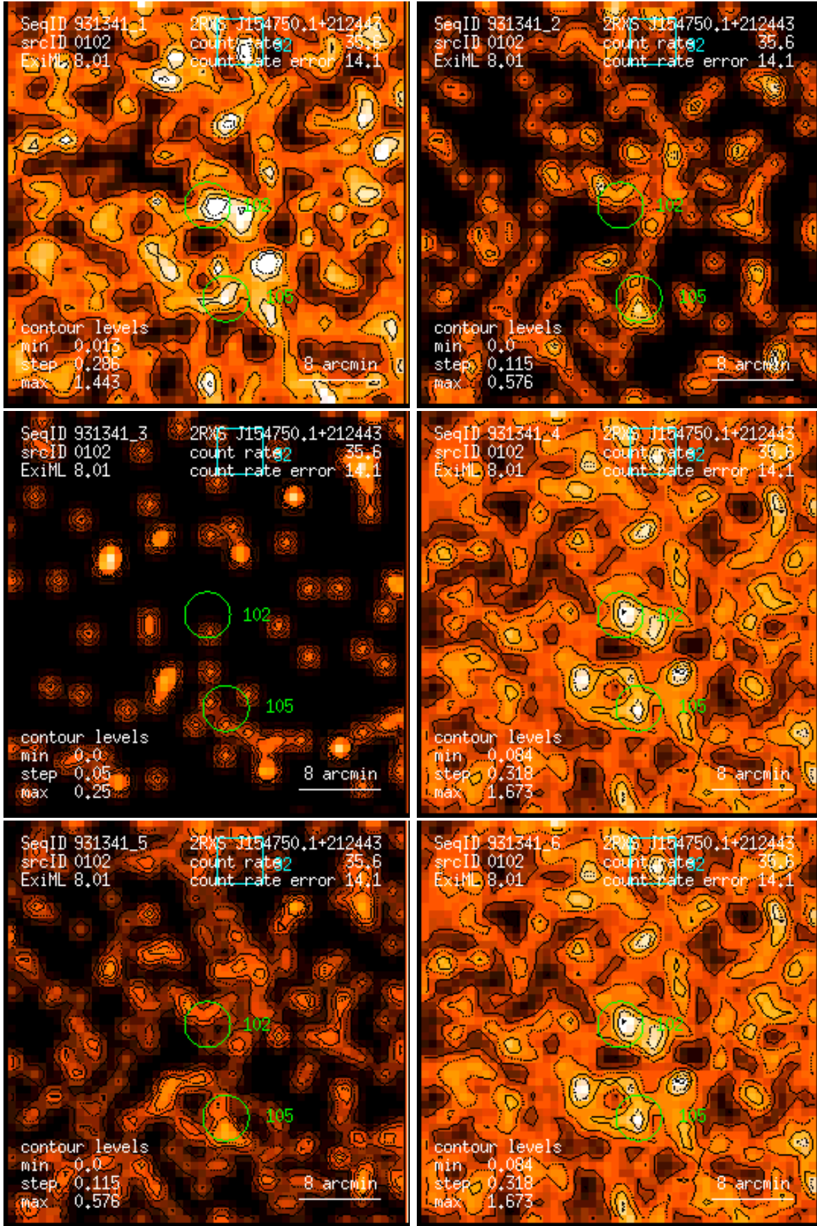
Figure 102: RASS 931341: detection 0102: band rate images, Gaussian filter: (1) PSPC channels 11 – 41, (2) 52 – 90, (3) 91 – 201, (4) 11 – 235, (5) 52 – 201, (6) 11 – 201. Broad band rates in counts/ks. Band rate contour levels in counts/ks/arcmin 2 .
