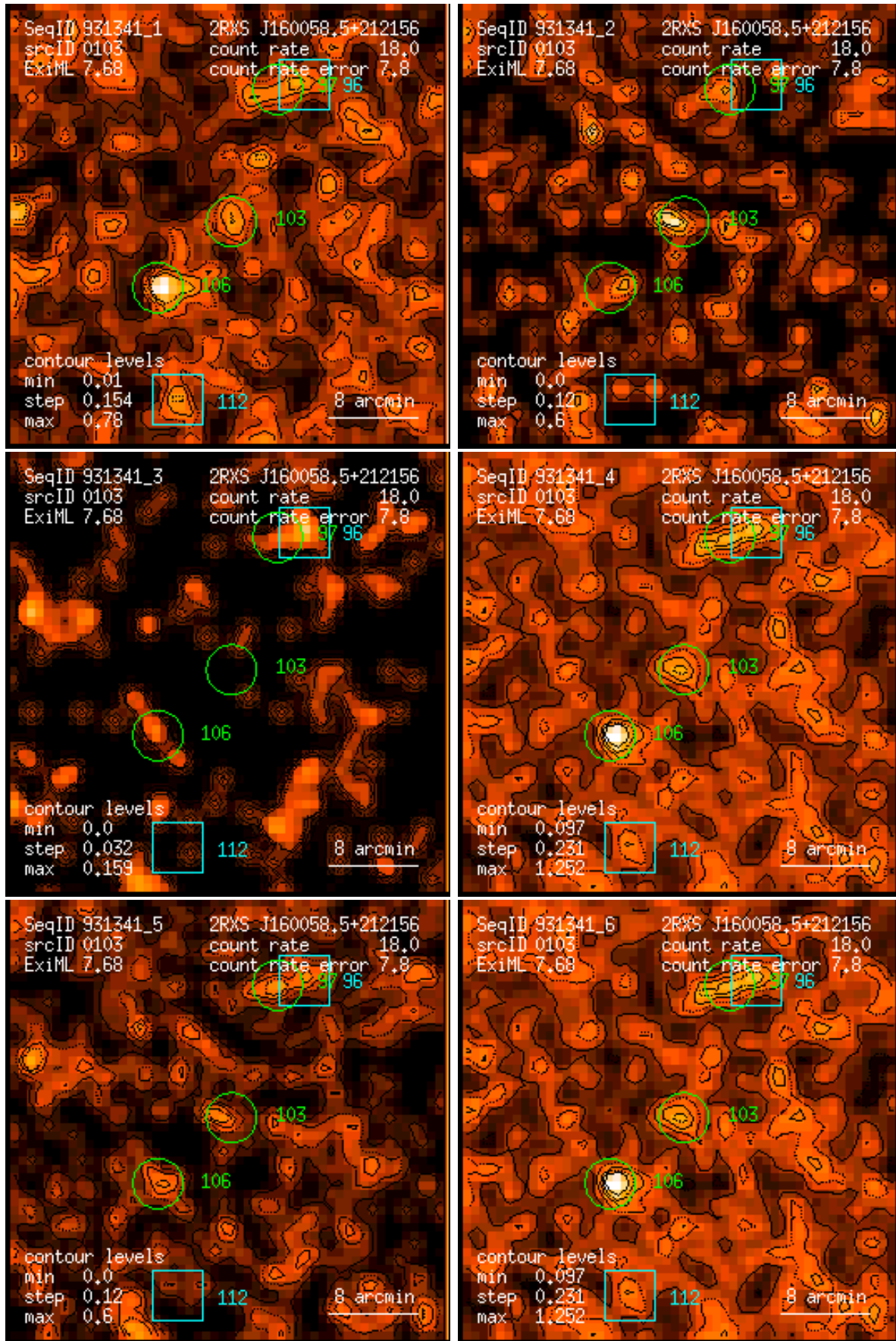
Figure 103: RASS 931341: detection 0103: band rate images, Gaussian filter: (1) PSPC channels 11 – 41, (2) 52 – 90, (3) 91 – 201, (4) 11 – 235, (5) 52 – 201, (6) 11 – 201. Broad band rates in counts/ks. Band rate contour levels in counts/ks/arcmin 2 .
