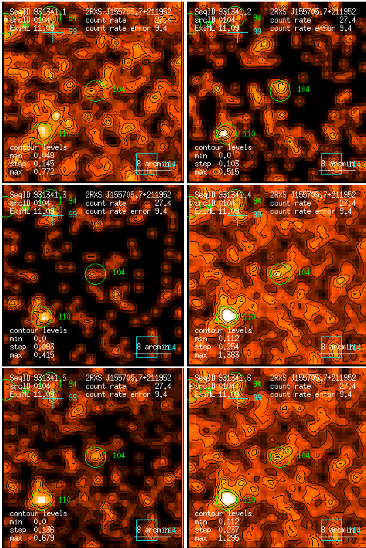
Figure 104: RASS 931341: detection 0104: band rate images, Gaussian filter: (1) PSPC channels 11 – 41, (2) 52 – 90, (3) 91 – 201, (4) 11 – 235, (5) 52 – 201, (6) 11 – 201. Broad band rates in counts/ks. Band rate contour levels in counts/ks/arcmin 2 .
