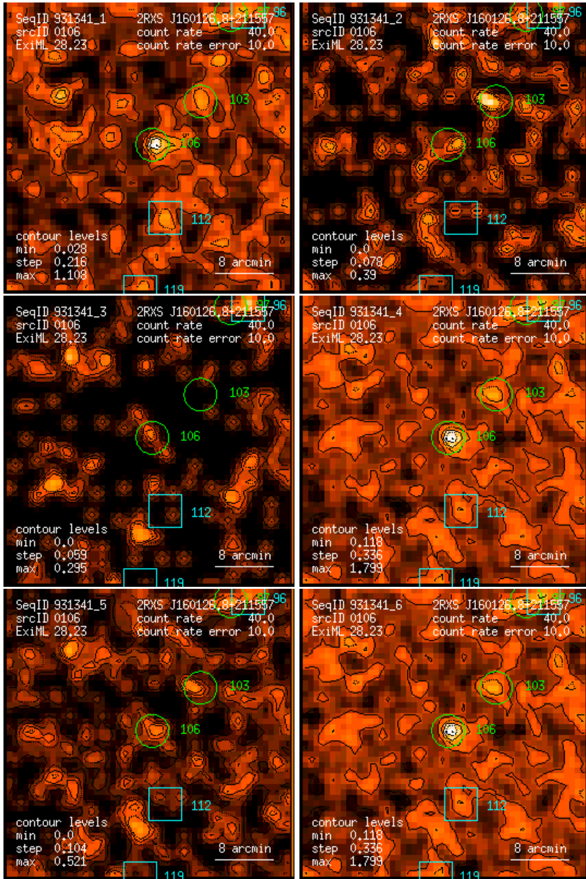
Figure 106: RASS 931341: detection 0106: band rate images, Gaussian filter: (1) PSPC channels 11 – 41, (2) 52 – 90, (3) 91 – 201, (4) 11 – 235, (5) 52 – 201, (6) 11 – 201. Broad band rates in counts/ks. Band rate contour levels in counts/ks/arcmin 2 .
