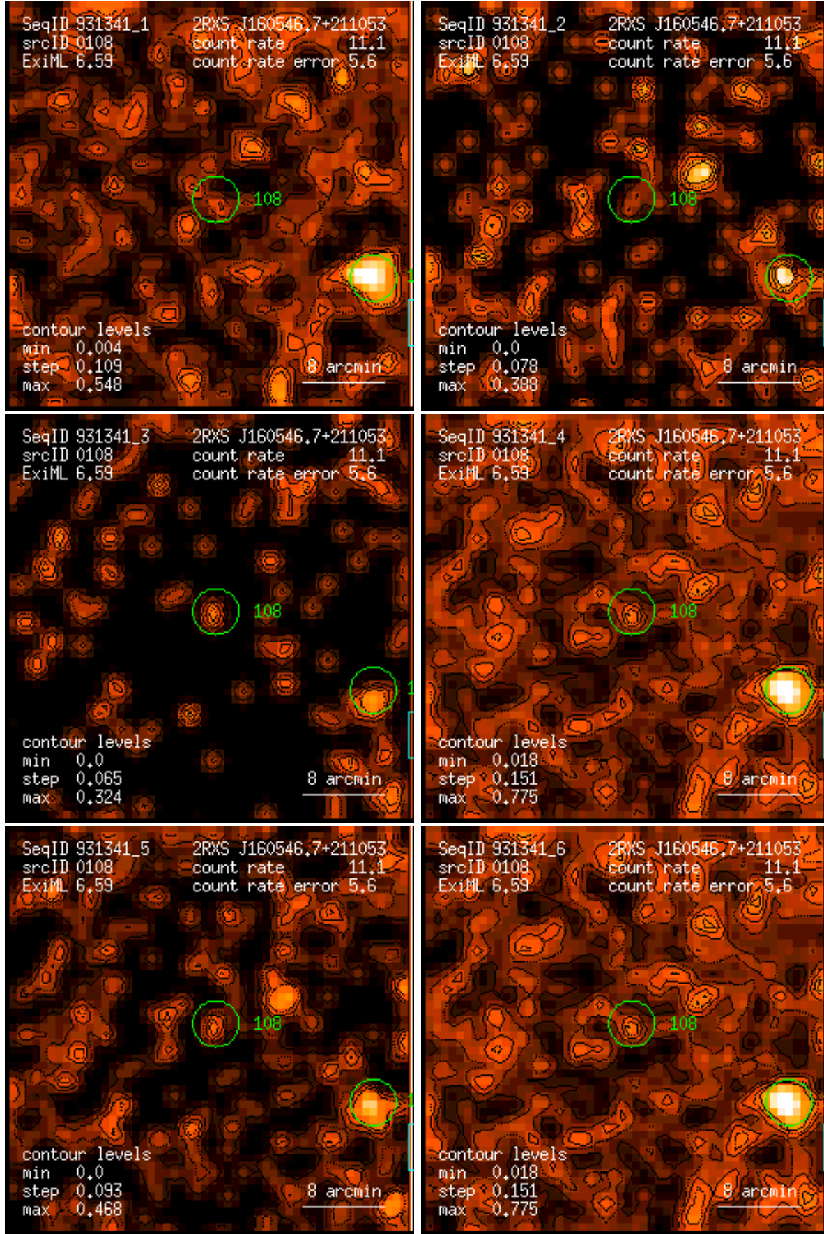
Figure 108: RASS 931341: detection 0108: band rate images, Gaussian filter: (1) PSPC channels 11 – 41, (2) 52 – 90, (3) 91 – 201, (4) 11 – 235, (5) 52 – 201, (6) 11 – 201. Broad band rates in counts/ks. Band rate contour levels in counts/ks/arcmin 2 .
