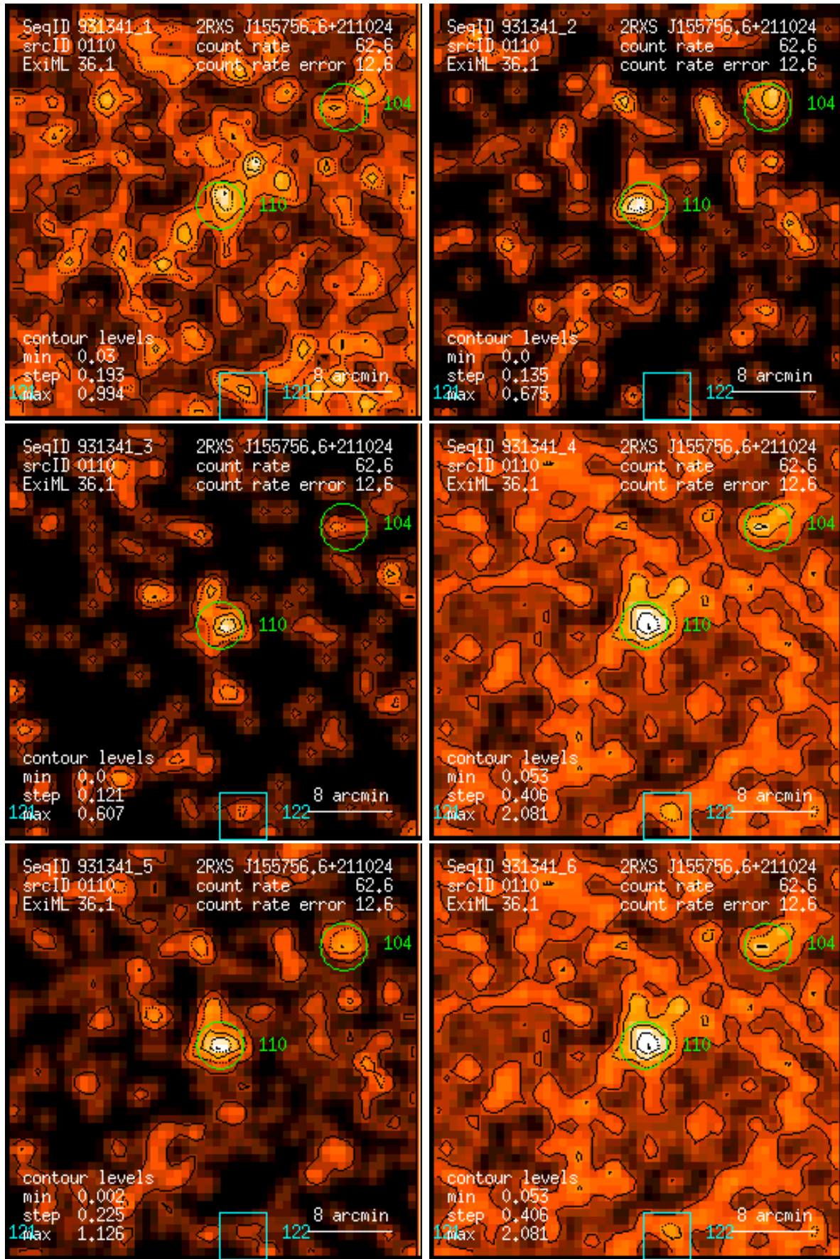
Figure 110: RASS 931341: detection 0110: band rate images, Gaussian filter: (1) PSPC channels 11 – 41, (2) 52 – 90, (3) 91 – 201, (4) 11 – 235, (5) 52 – 201, (6) 11 – 201. Broad band rates in counts/ks. Band rate contour levels in counts/ks/arcmin 2 .
