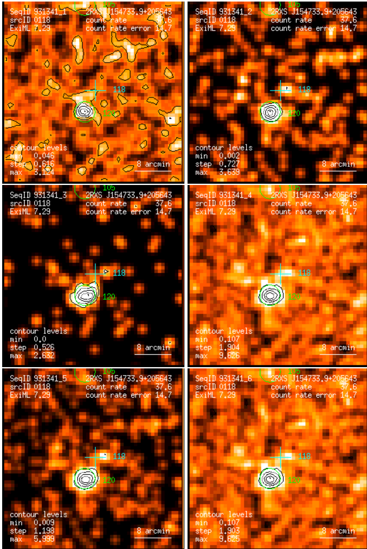
Figure 118: RASS 931341: detection 0118: band rate images, Gaussian filter: (1) PSPC channels 11 – 41, (2) 52 – 90, (3) 91 – 201, (4) 11 – 235, (5) 52 – 201, (6) 11 – 201. Broad band rates in counts/ks. Band rate contour levels in counts/ks/arcmin 2 .
