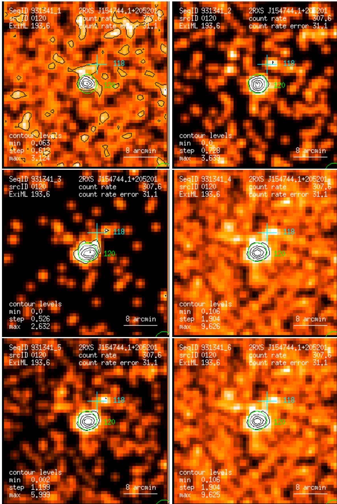
Figure 120: RASS 931341: detection 0120: band rate images, Gaussian filter: (1) PSPC channels 11 – 41, (2) 52 – 90, (3) 91 – 201, (4) 11 – 235, (5) 52 – 201, (6) 11 – 201. Broad band rates in counts/ks. Band rate contour levels in counts/ks/arcmin 2 .
