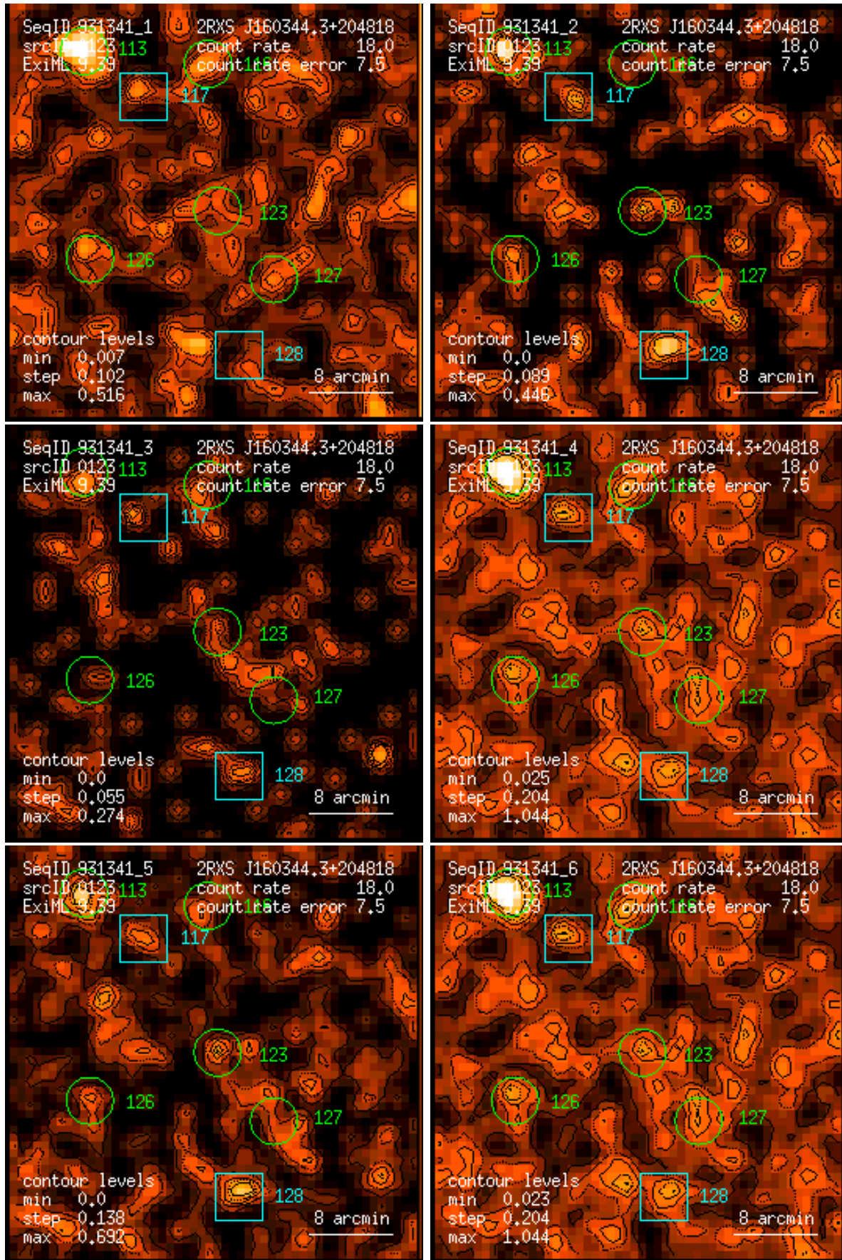
Figure 123: RASS 931341: detection 0123: band rate images, Gaussian filter: (1) PSPC channels 11 – 41, (2) 52 – 90, (3) 91 – 201, (4) 11 – 235, (5) 52 – 201, (6) 11 – 201. Broad band rates in counts/ks. Band rate contour levels in counts/ks/arcmin 2 .
