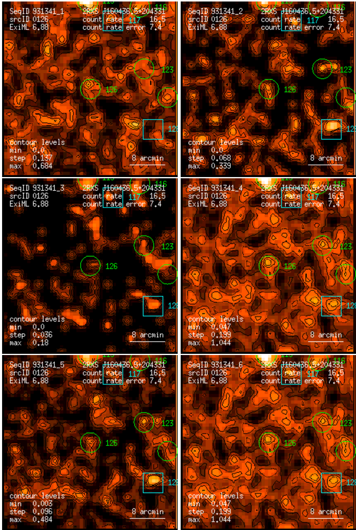
Figure 126: RASS 931341: detection 0126: band rate images, Gaussian filter: (1) PSPC channels 11 – 41, (2) 52 – 90, (3) 91 – 201, (4) 11 – 235, (5) 52 – 201, (6) 11 – 201. Broad band rates in counts/ks. Band rate contour levels in counts/ks/arcmin 2 .
