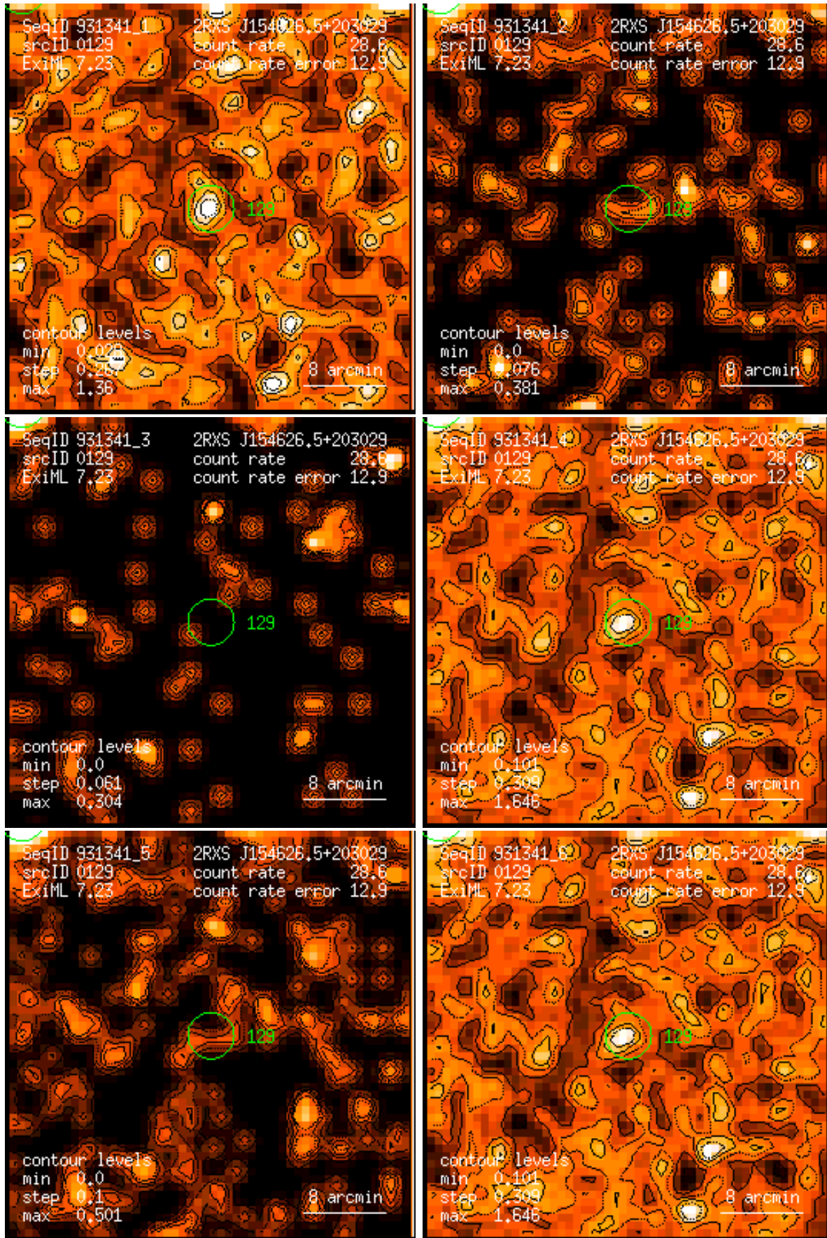
Figure 129: RASS 931341: detection 0129: band rate images, Gaussian filter: (1) PSPC channels 11 – 41, (2) 52 – 90, (3) 91 – 201, (4) 11 – 235, (5) 52 – 201, (6) 11 – 201. Broad band rates in counts/ks. Band rate contour levels in counts/ks/arcmin 2 .
