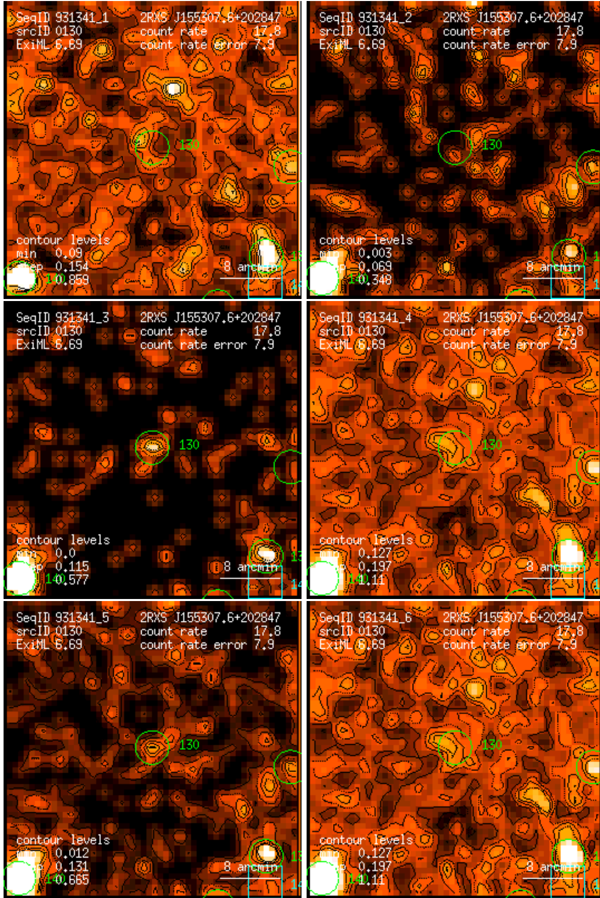
Figure 130: RASS 931341: detection 0130: band rate images, Gaussian filter: (1) PSPC channels 11 – 41, (2) 52 – 90, (3) 91 – 201, (4) 11 – 235, (5) 52 – 201, (6) 11 – 201. Broad band rates in counts/ks. Band rate contour levels in counts/ks/arcmin 2 .
