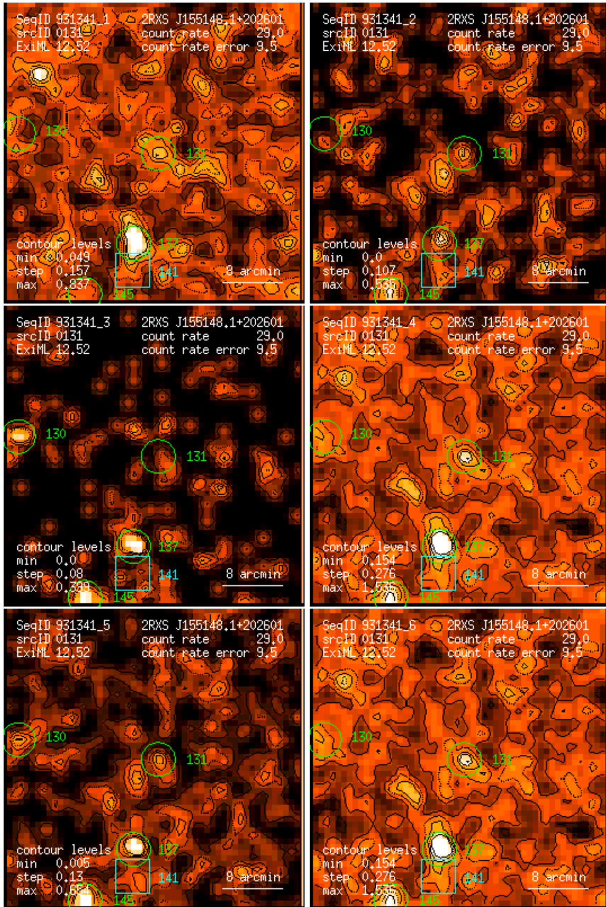
Figure 131: RASS 931341: detection 0131: band rate images, Gaussian filter: (1) PSPC channels 11 – 41, (2) 52 – 90, (3) 91 – 201, (4) 11 – 235, (5) 52 – 201, (6) 11 – 201. Broad band rates in counts/ks. Band rate contour levels in counts/ks/arcmin 2 .
