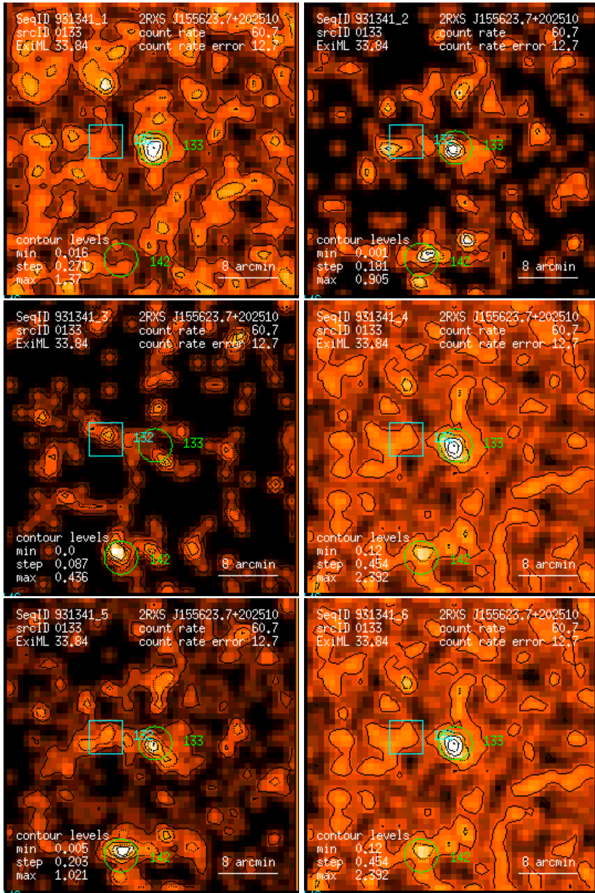
Figure 133: RASS 931341: detection 0133: band rate images, Gaussian filter: (1) PSPC channels 11 – 41, (2) 52 – 90, (3) 91 – 201, (4) 11 – 235, (5) 52 – 201, (6) 11 – 201. Broad band rates in counts/ks. Band rate contour levels in counts/ks/arcmin 2 .
