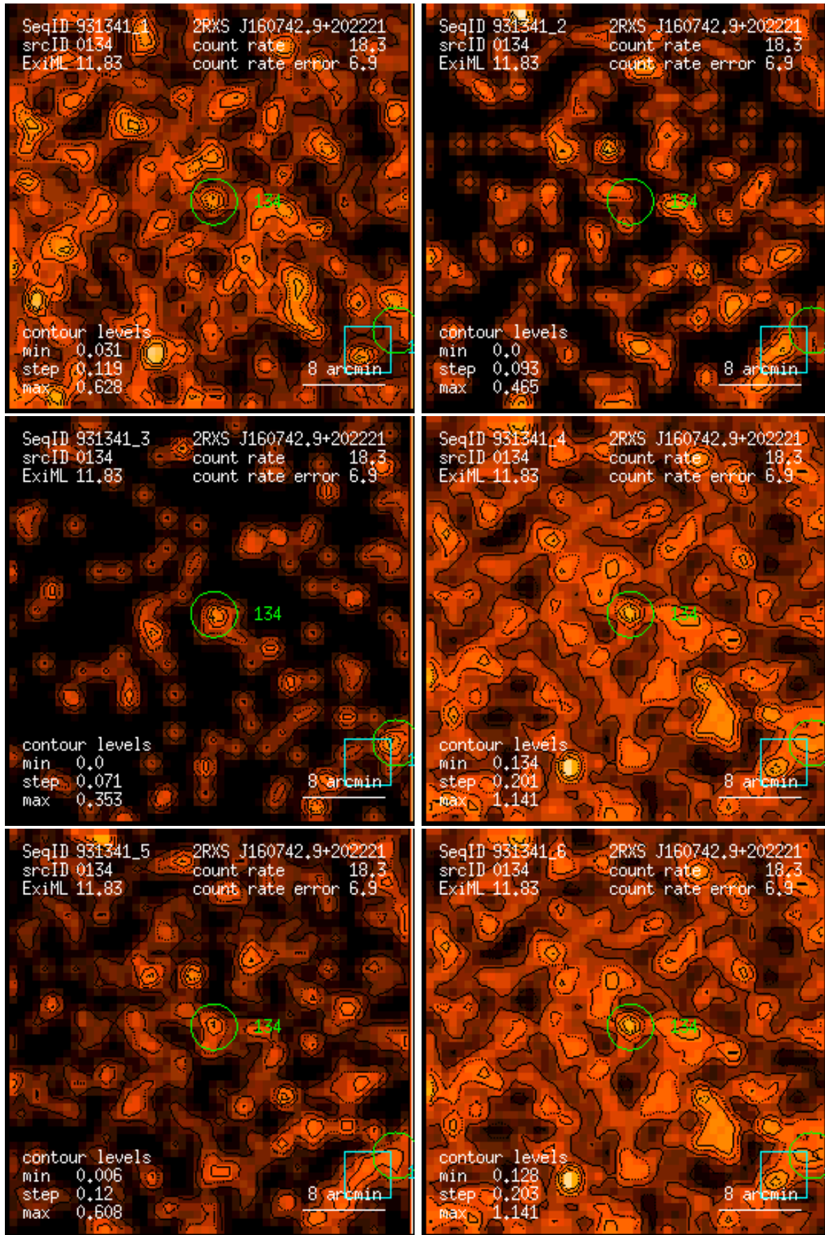
Figure 134: RASS 931341: detection 0134: band rate images, Gaussian filter: (1) PSPC channels 11 – 41, (2) 52 – 90, (3) 91 – 201, (4) 11 – 235, (5) 52 – 201, (6) 11 – 201. Broad band rates in counts/ks. Band rate contour levels in counts/ks/arcmin 2 .
