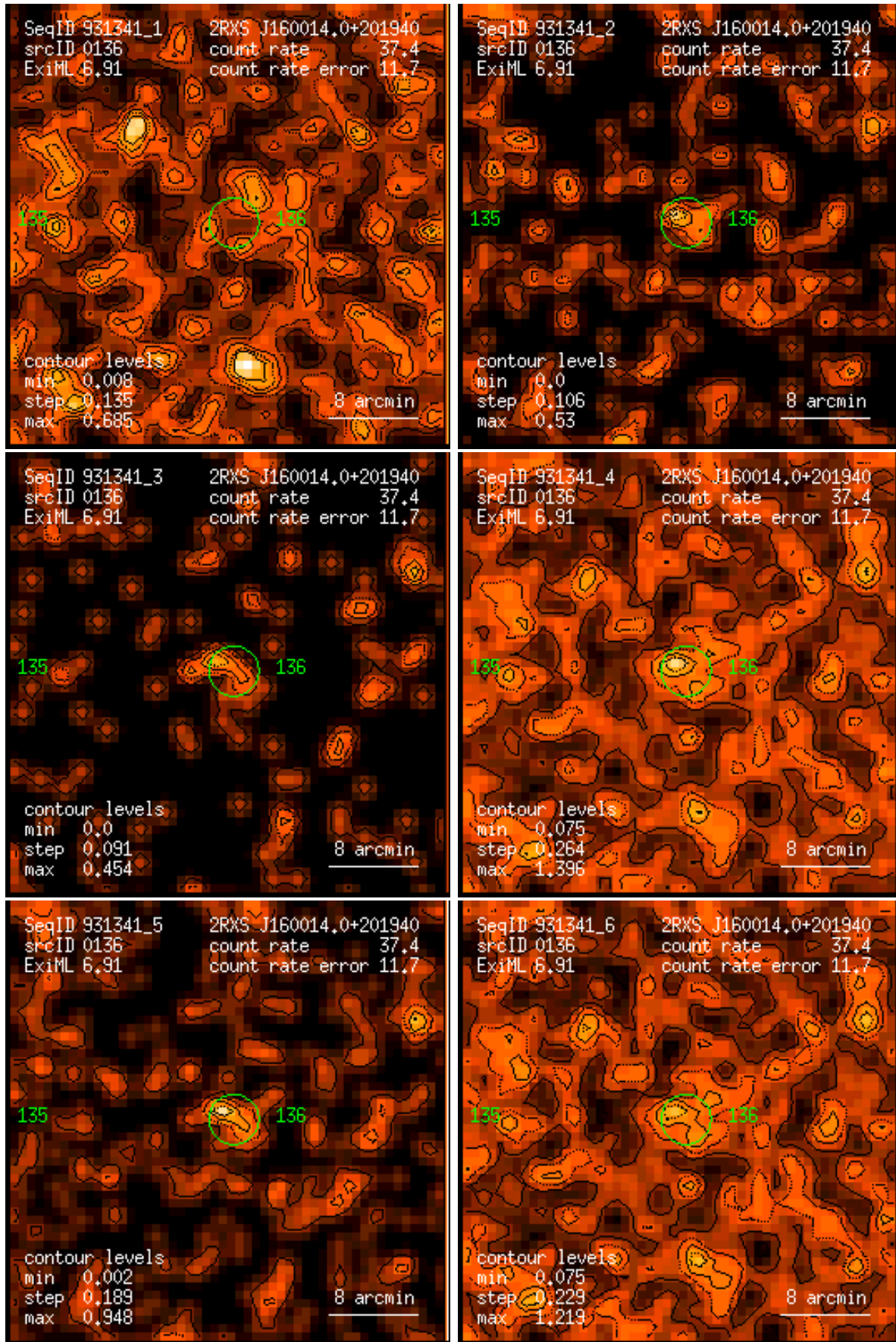
Figure 136: RASS 931341: detection 0136: band rate images, Gaussian filter: (1) PSPC channels 11 – 41, (2) 52 – 90, (3) 91 – 201, (4) 11 – 235, (5) 52 – 201, (6) 11 – 201. Broad band rates in counts/ks. Band rate contour levels in counts/ks/arcmin 2 .
