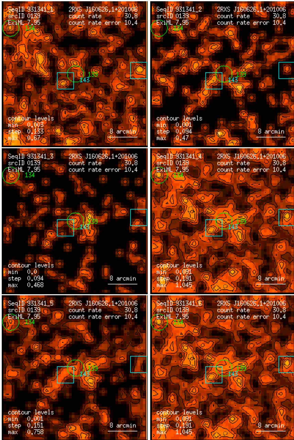
Figure 139: RASS 931341: detection 0139: band rate images, Gaussian filter: (1) PSPC channels 11 – 41, (2) 52 – 90, (3) 91 – 201, (4) 11 – 235, (5) 52 – 201, (6) 11 – 201. Broad band rates in counts/ks. Band rate contour levels in counts/ks/arcmin 2 .
