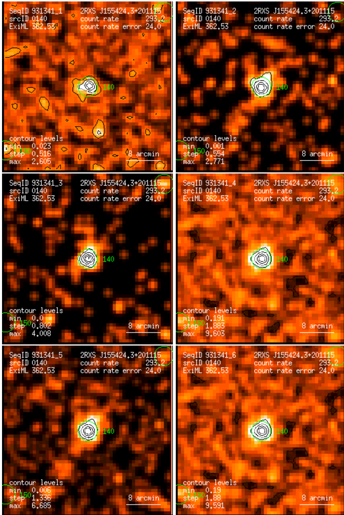
Figure 140: RASS 931341: detection 0140: band rate images, Gaussian filter: (1) PSPC channels 11 – 41, (2) 52 – 90, (3) 91 – 201, (4) 11 – 235, (5) 52 – 201, (6) 11 – 201. Broad band rates in counts/ks. Band rate contour levels in counts/ks/arcmin 2 .
