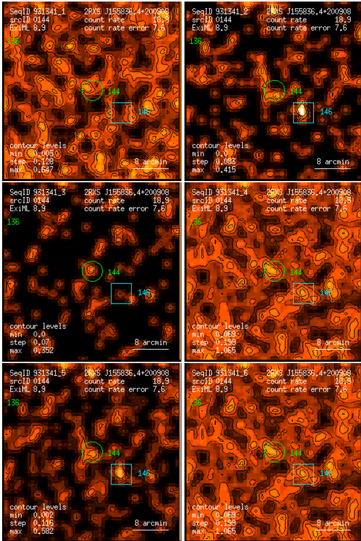
Figure 144: RASS 931341: detection 0144: band rate images, Gaussian filter: (1) PSPC channels 11 – 41, (2) 52 – 90, (3) 91 – 201, (4) 11 – 235, (5) 52 – 201, (6) 11 – 201. Broad band rates in counts/ks. Band rate contour levels in counts/ks/arcmin 2 .
